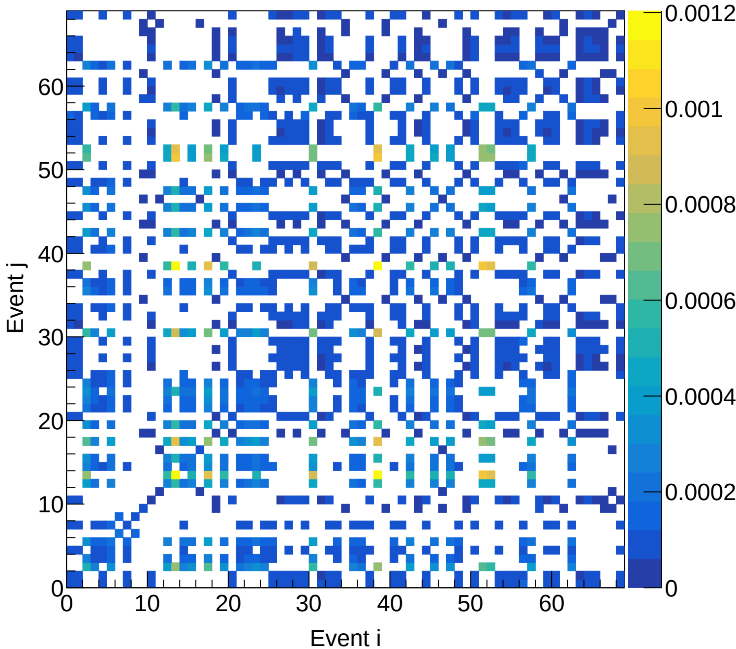
LD2 (total) Covariance | M: [6.0, 6.3] xF: [0.40, 0.45)
