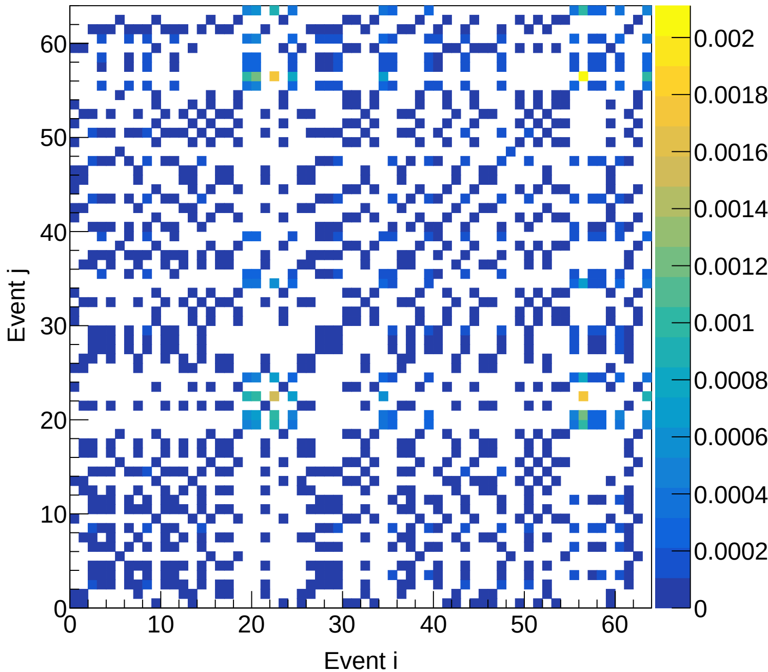
LH2 (mix) Covariance | M: [4.2, 4.5) xF: [0.45, 0.50)
