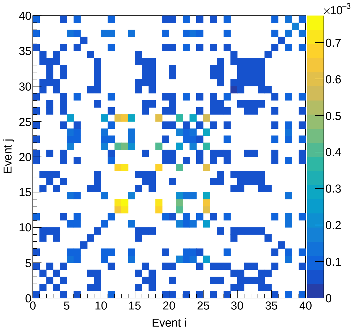
LH2 (mix) Covariance | M: [4.2, 4.5) xF: [0.50, 0.55)
