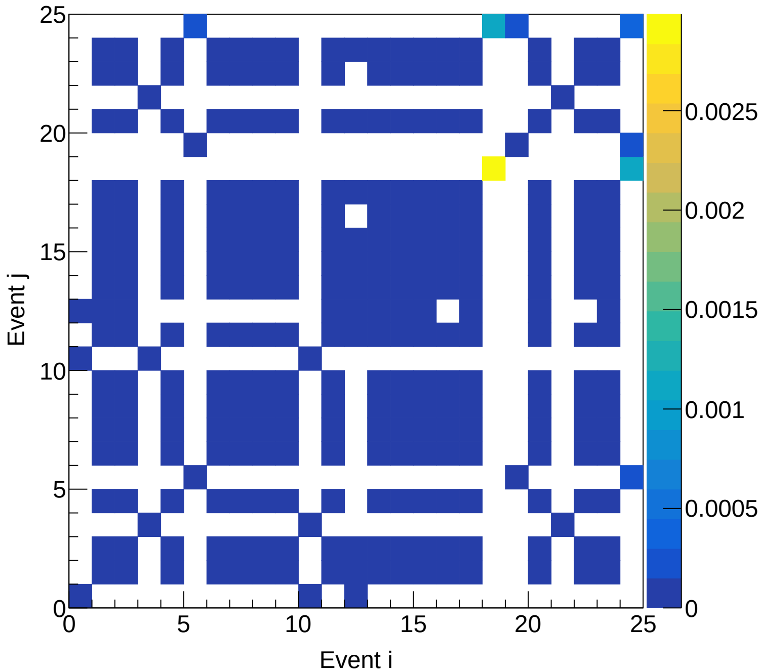
LH2 (mix) Covariance | M: [4.5, 4.8) xF: [0.50, 0.55)
