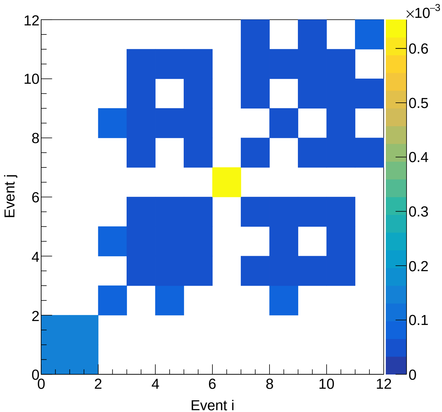
LH2 (mix) Covariance | M: [4.8, 5.1] xF: [0.50, 0.55]
