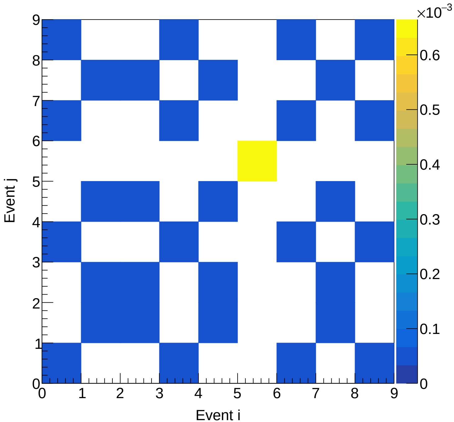
LH2 (mix) Covariance | M: [5.1, 5.4) xF: [0.50, 0.55)
