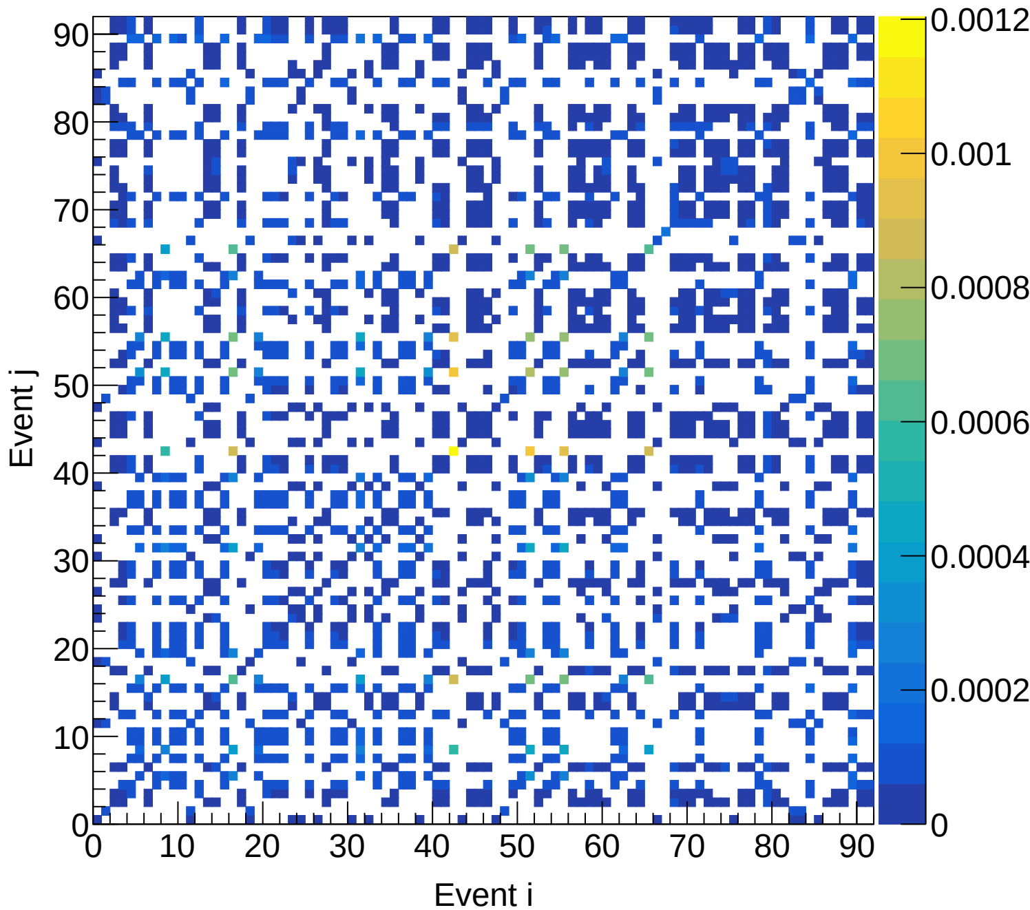
LH2 (mix) Covariance | M: [3.9, 4.2) xF: [0.55, 0.60)
