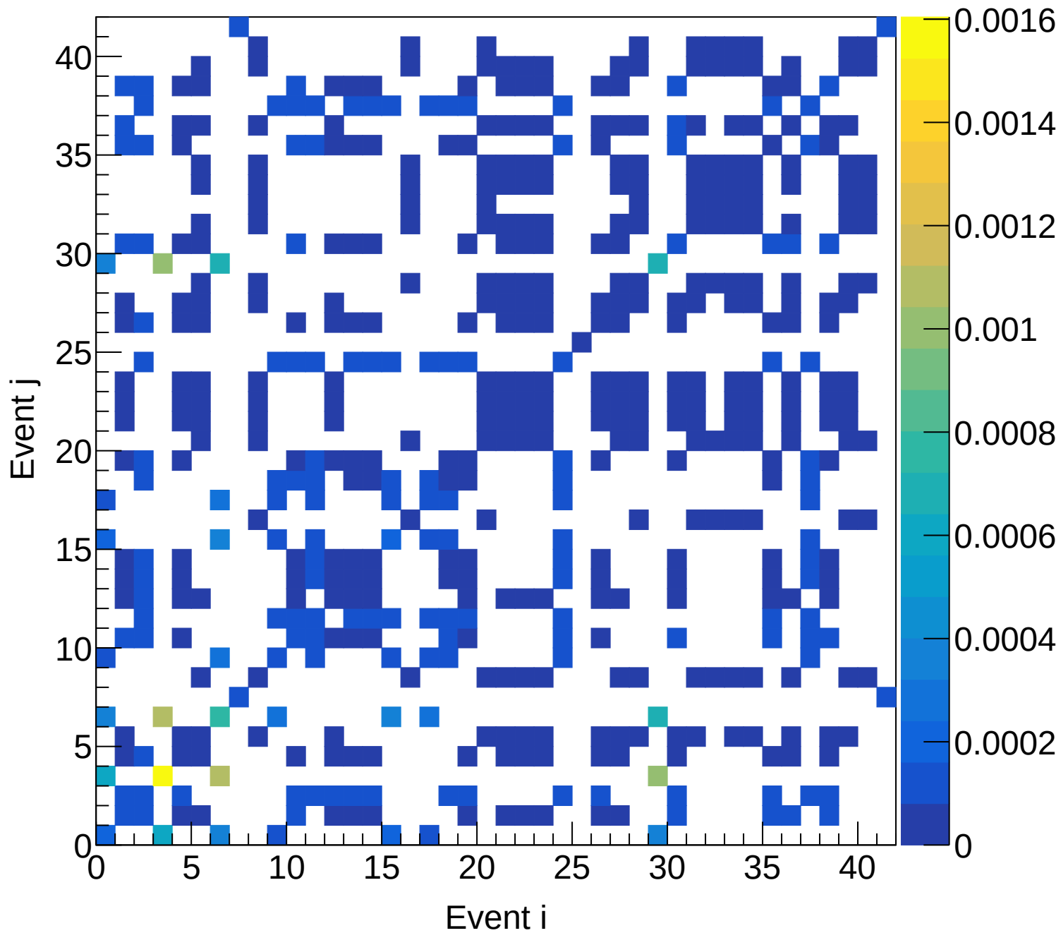
LH2 (mix) Covariance | M: [4.2, 4.5] xF: [0.55, 0.60)
