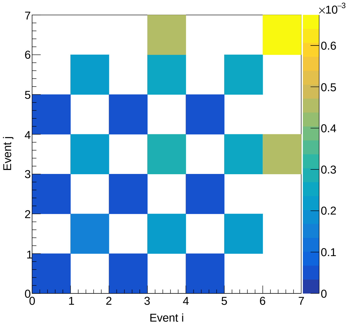
LH2 (mix) Covariance | M: [4.8, 5.1) xF: [0.55, 0.60)
