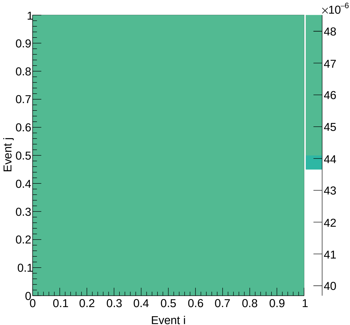
LH2 (mix) Covariance | M: [6.0, 6.3) xF: [0.60, 0.65)
