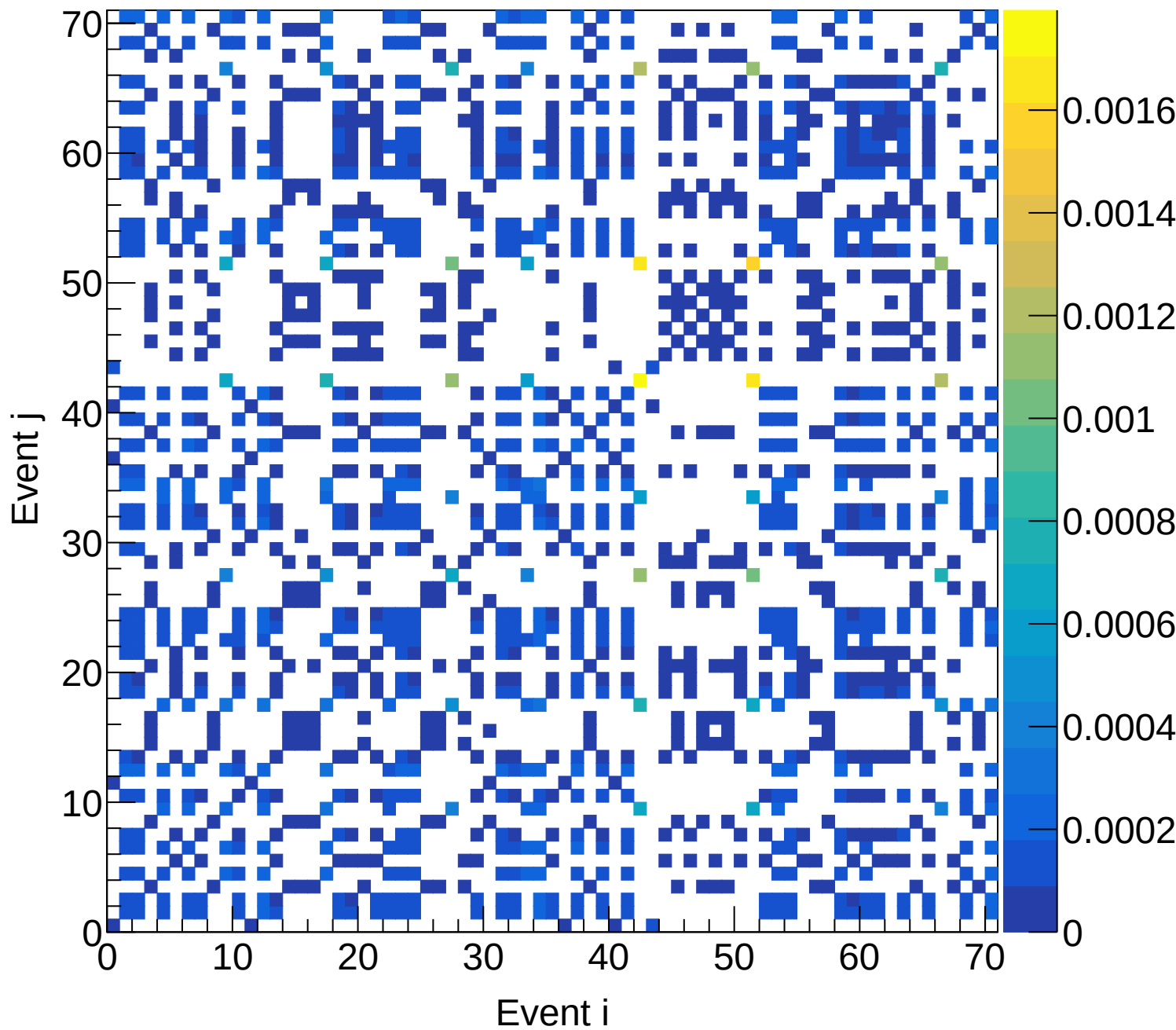
LH2 (mix) Covariance | M: [3.9, 4.2) xF: [0.60, 0.65)
