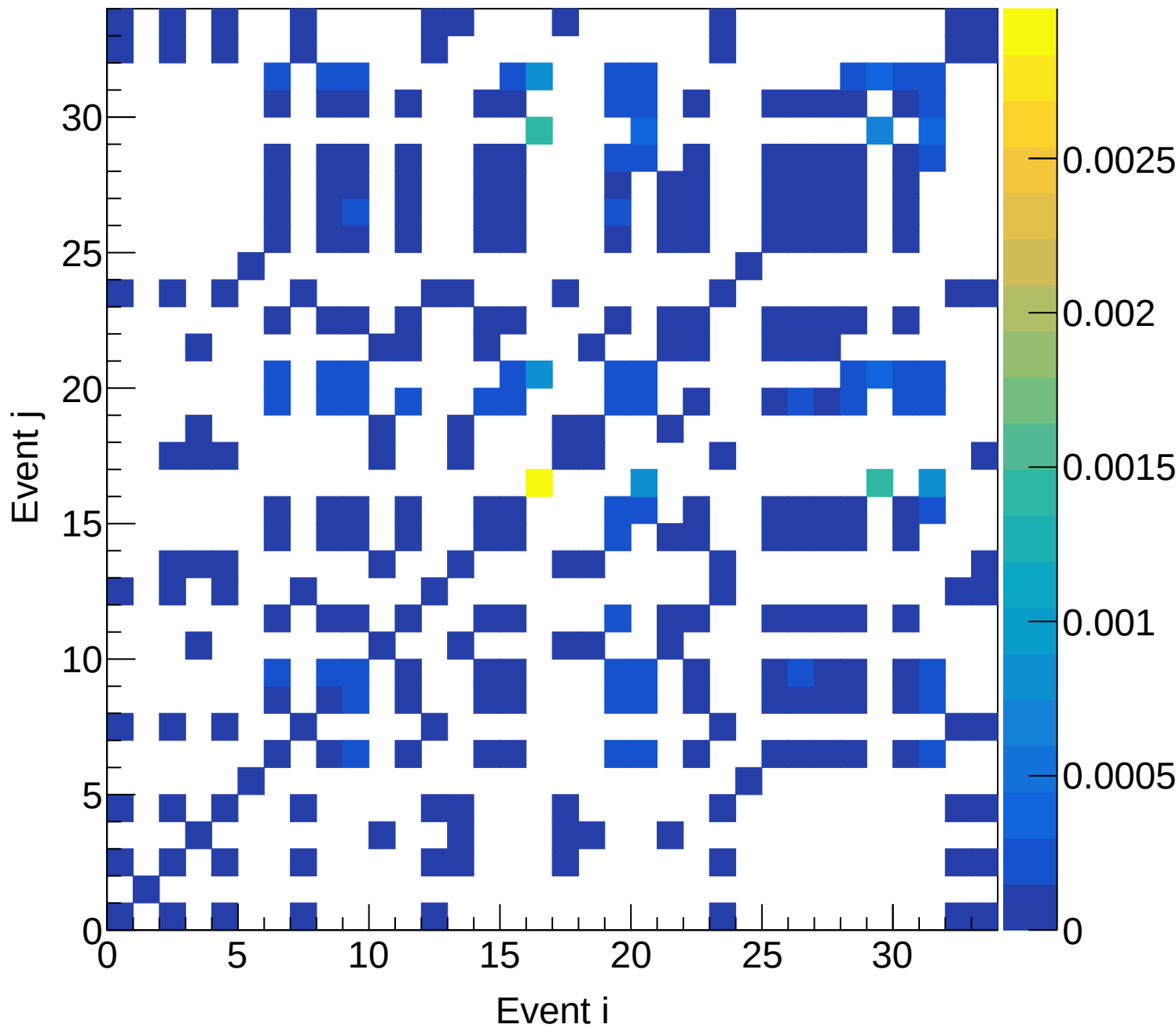
LH2 (mix) Covariance | M: [4.2, 4.5) xF: [0.60, 0.65)
