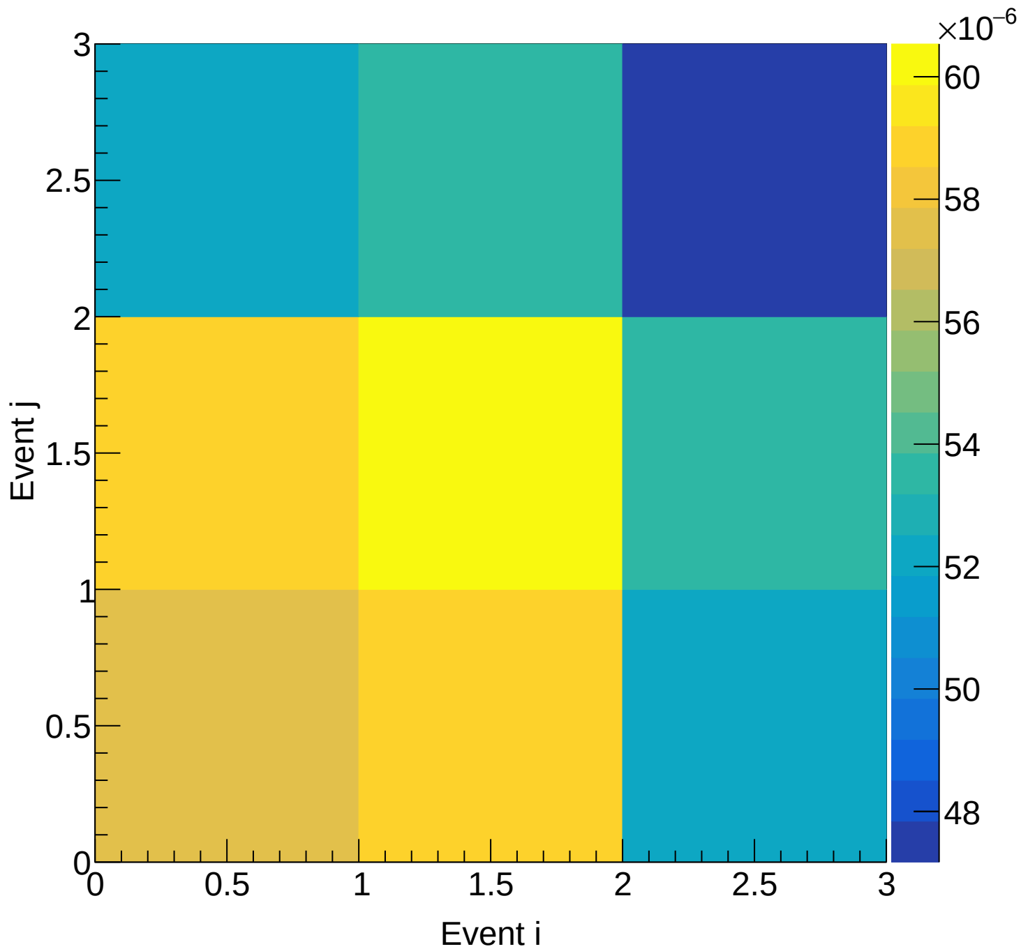
LH2 (mix) Covariance | M: [5.1, 5.4) xF: [0.60, 0.65)
