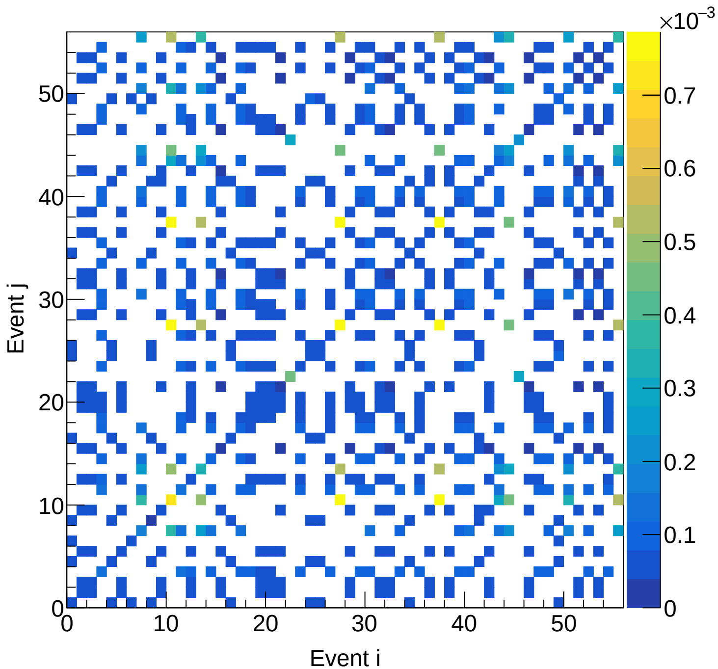
LH2 (mix) Covariance | M: [3.9, 4.2] xF: [0.65, 0.70)
