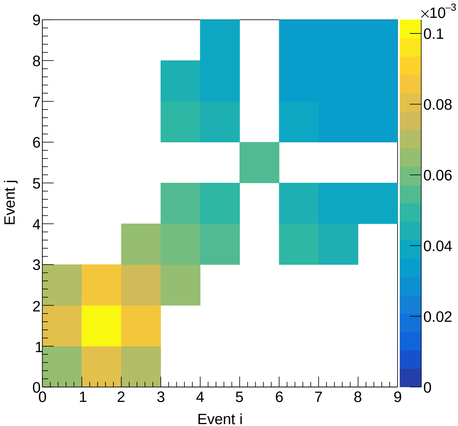
LH2 (mix) Covariance | M: [4.5, 4.8] xF: [0.65, 0.70]
