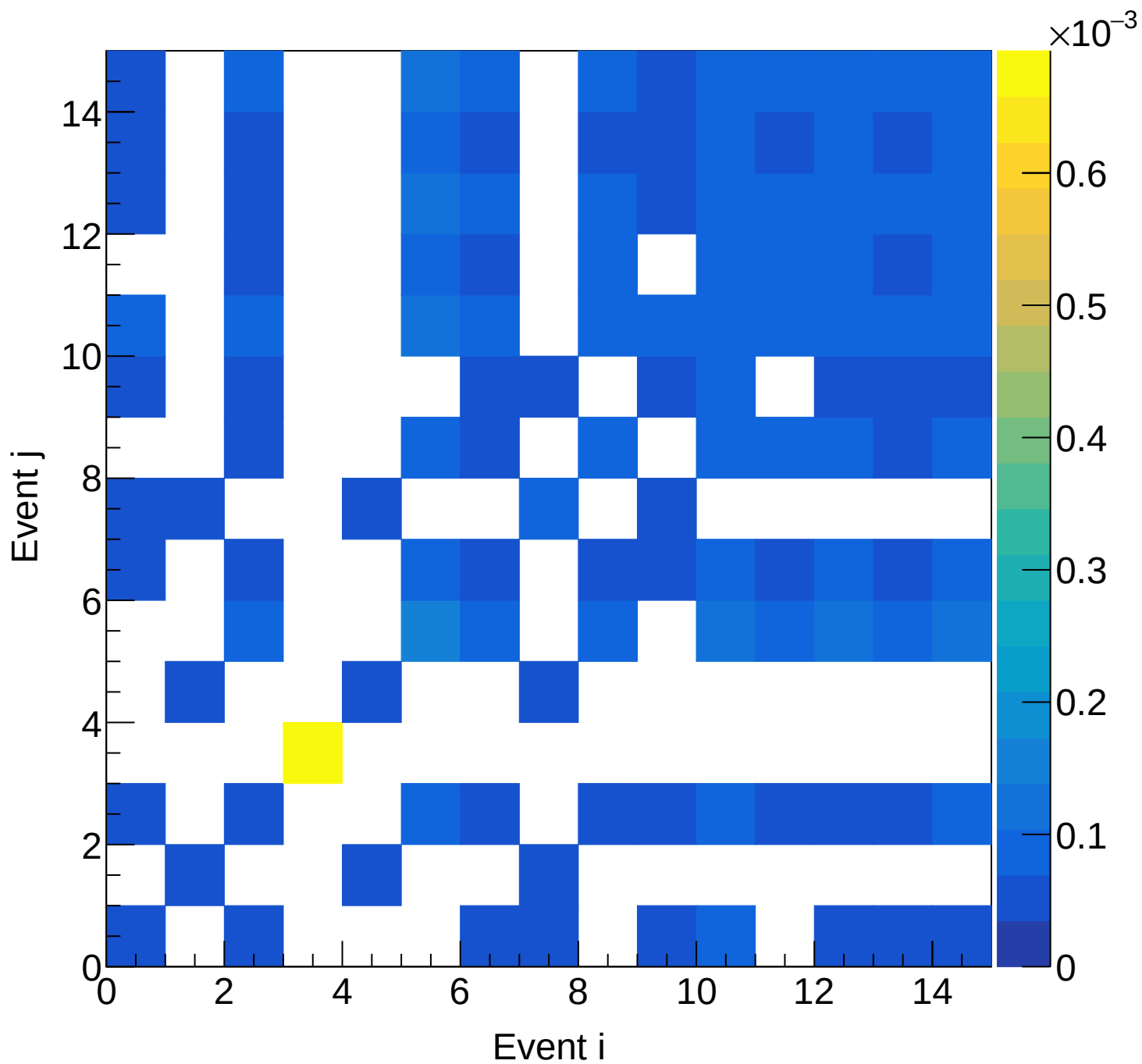
LH2 (mix) Covariance | M: [4.2, 4.5] xF: [0.70, 0.75]
