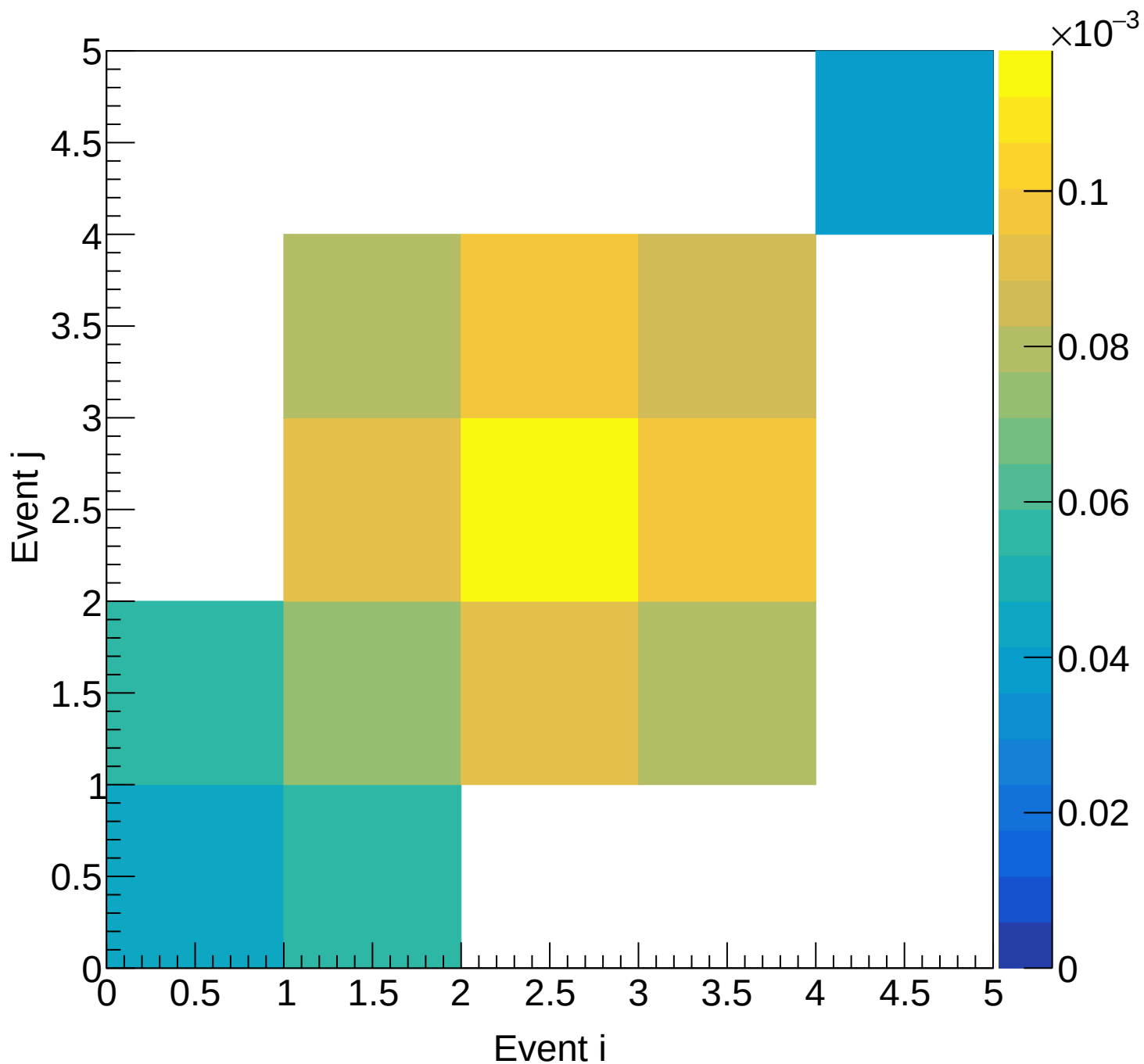
LH2 (mix) Covariance | M: [4.5, 4.8) xF: [0.70, 0.75)
