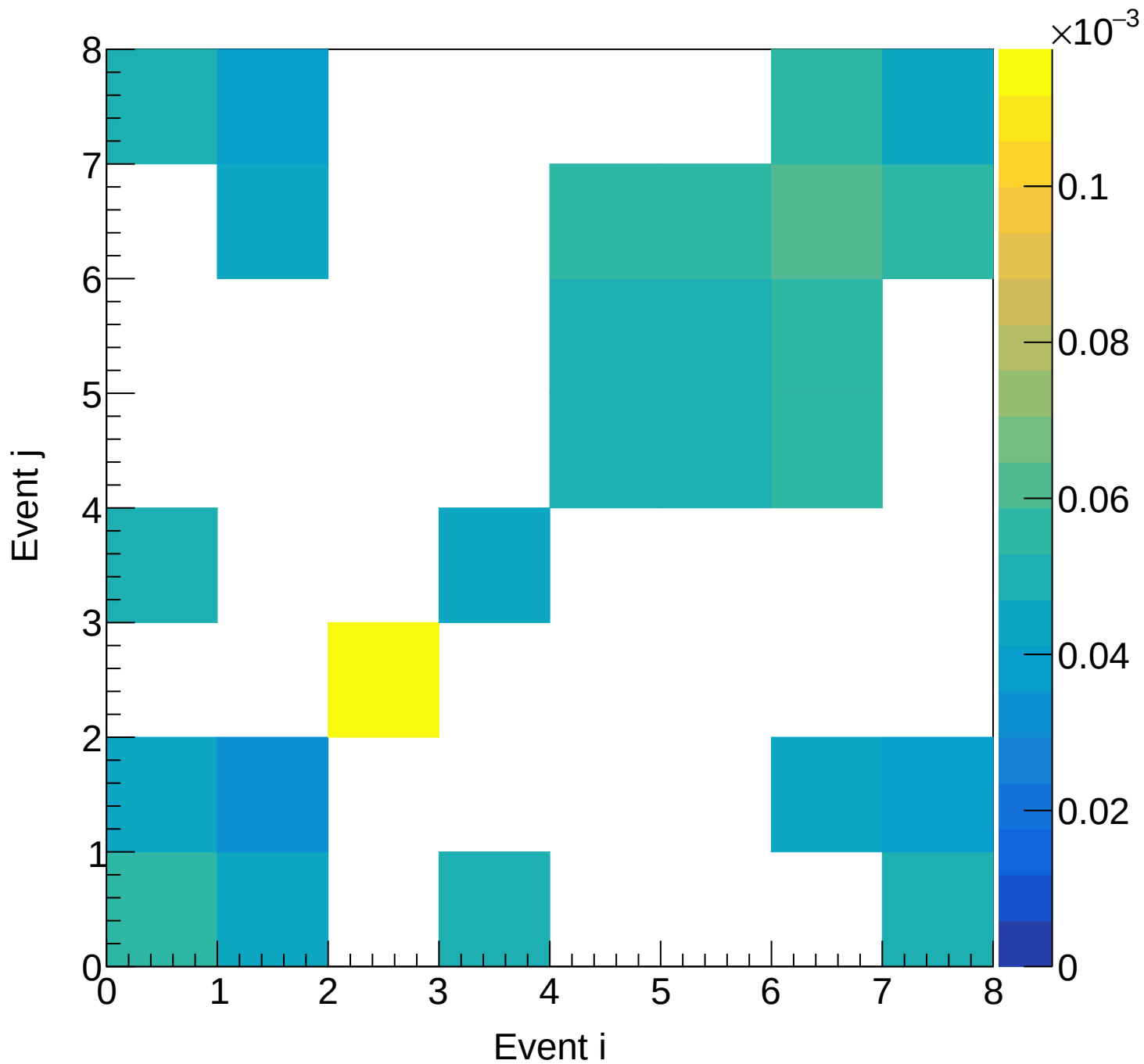
LH2 (mix) Covariance | M: [5.4, 5.7) xF: [0.00, 0.05)
