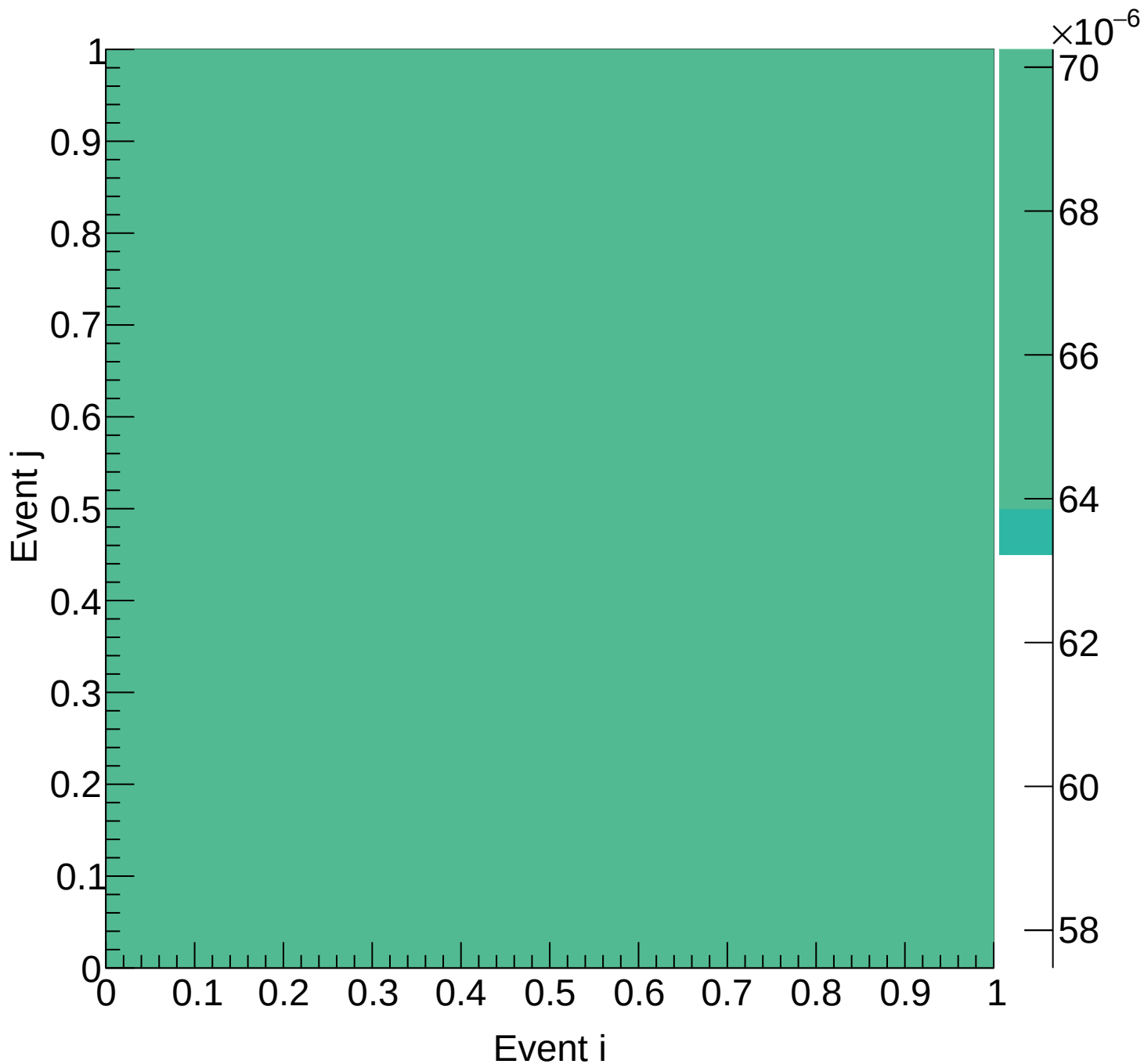
LH2 (mix) Covariance | M: [5.7, 6.0] xF: [0.00, 0.05)
