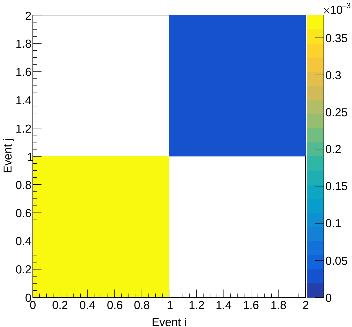
LH2 (mix) Covariance | M: [6.6, 6.9] xF: [0.05, 0.10)
