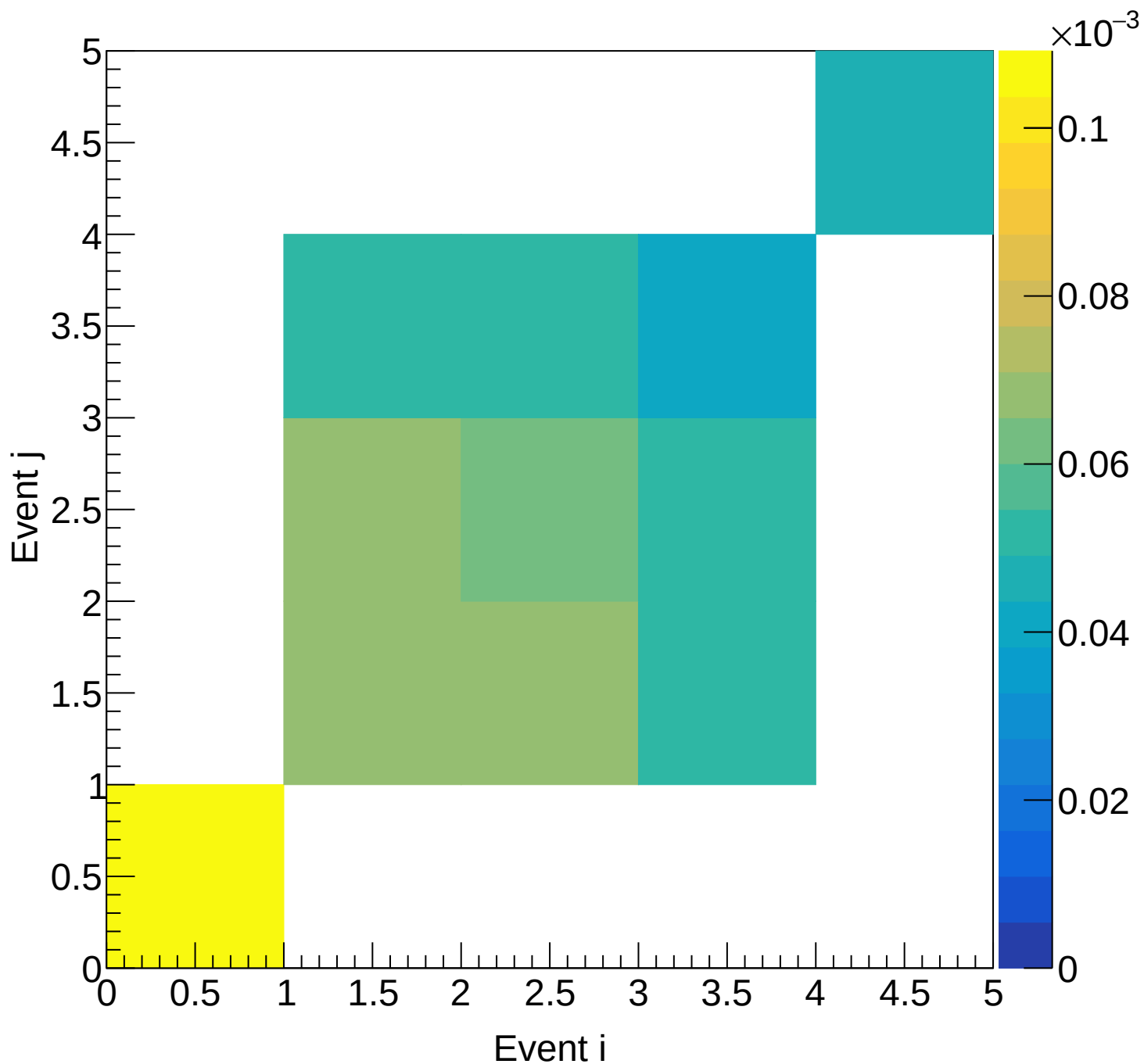
LH2 (mix) Covariance | M: [4.5, 4.8) xF: [0.05, 0.10)
