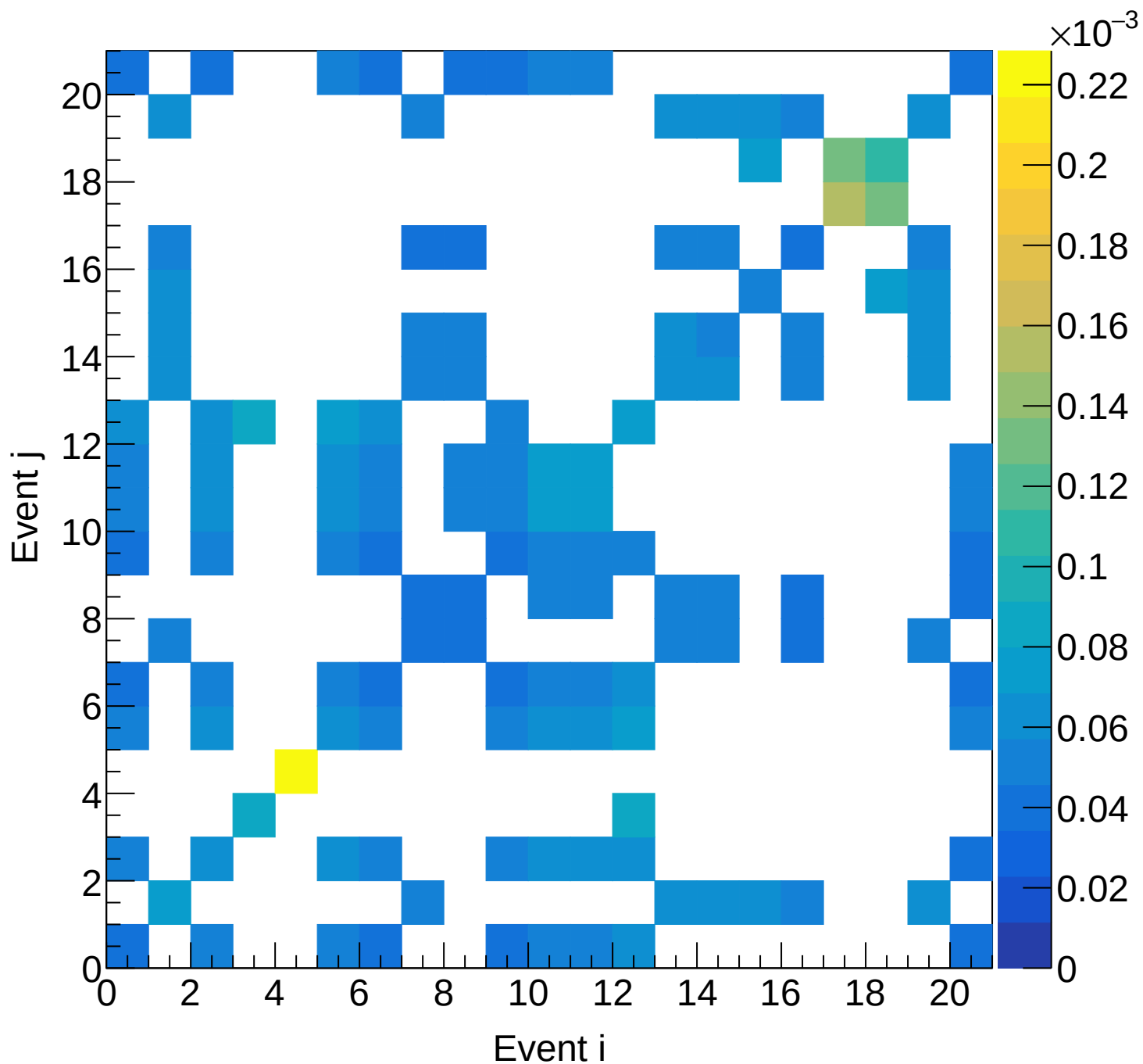
LH2 (mix) Covariance | M: [4.8, 5.1) xF: [0.05, 0.10)
