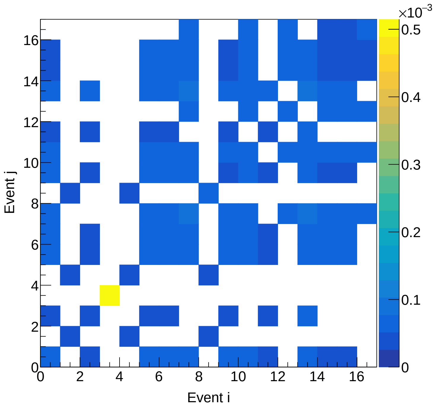
LH2 (mix) Covariance | M: [5.4, 5.7) xF: [0.05, 0.10)
