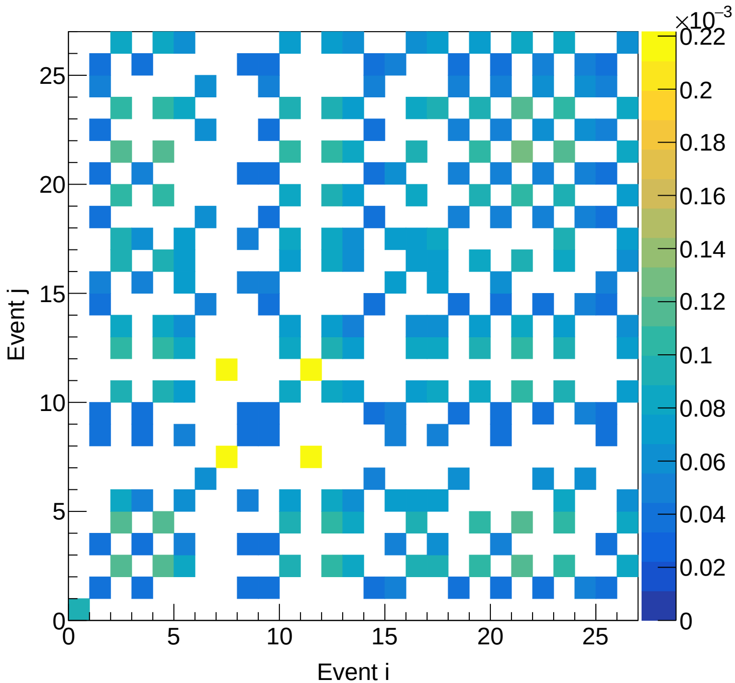
LH2 (mix) Covariance | M: [4.2, 4.5] xF: [0.15, 0.20]
