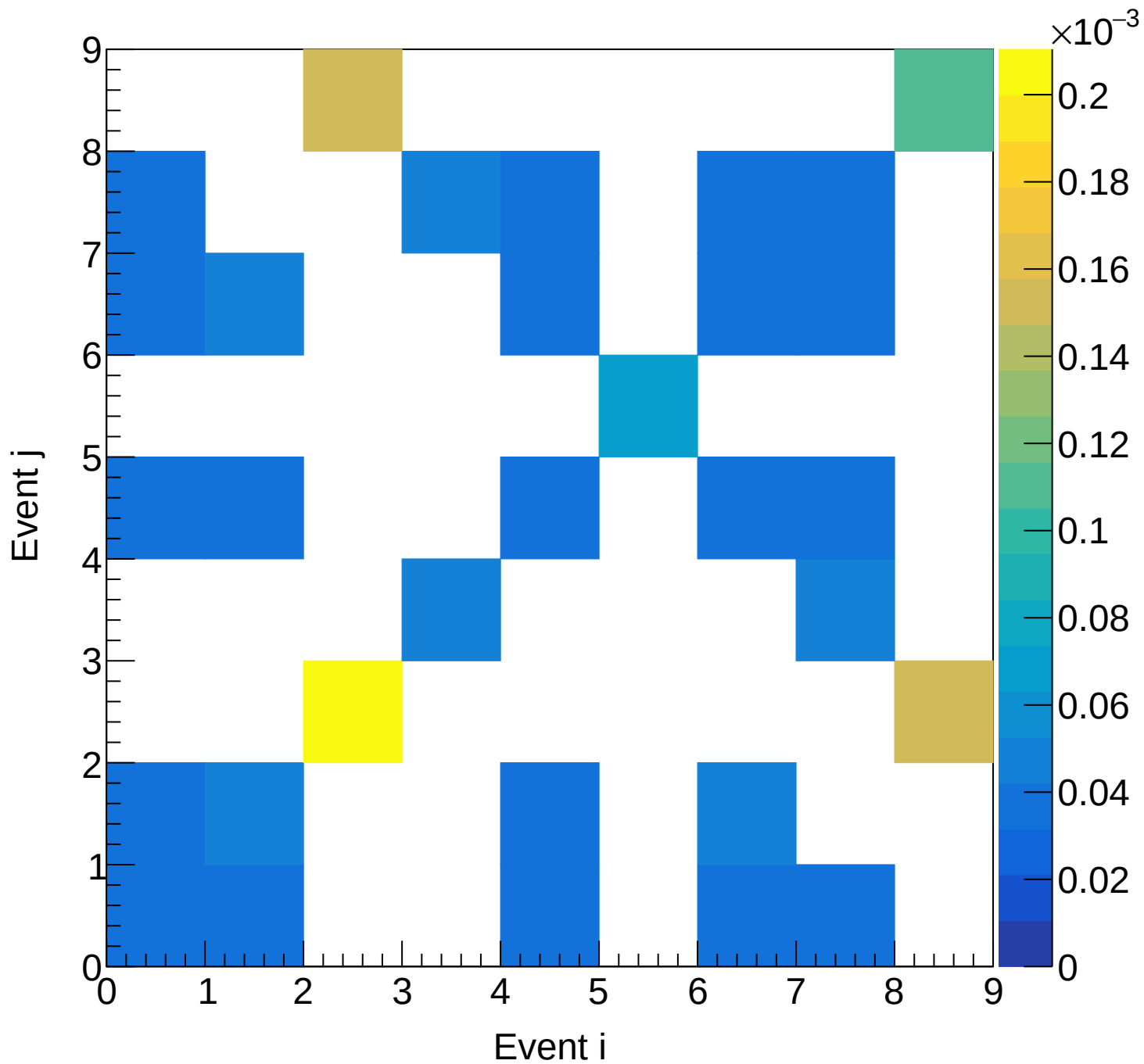
LH2 (mix) Covariance | M: [4.2, 4.5] xF: [0.10, 0.15]
