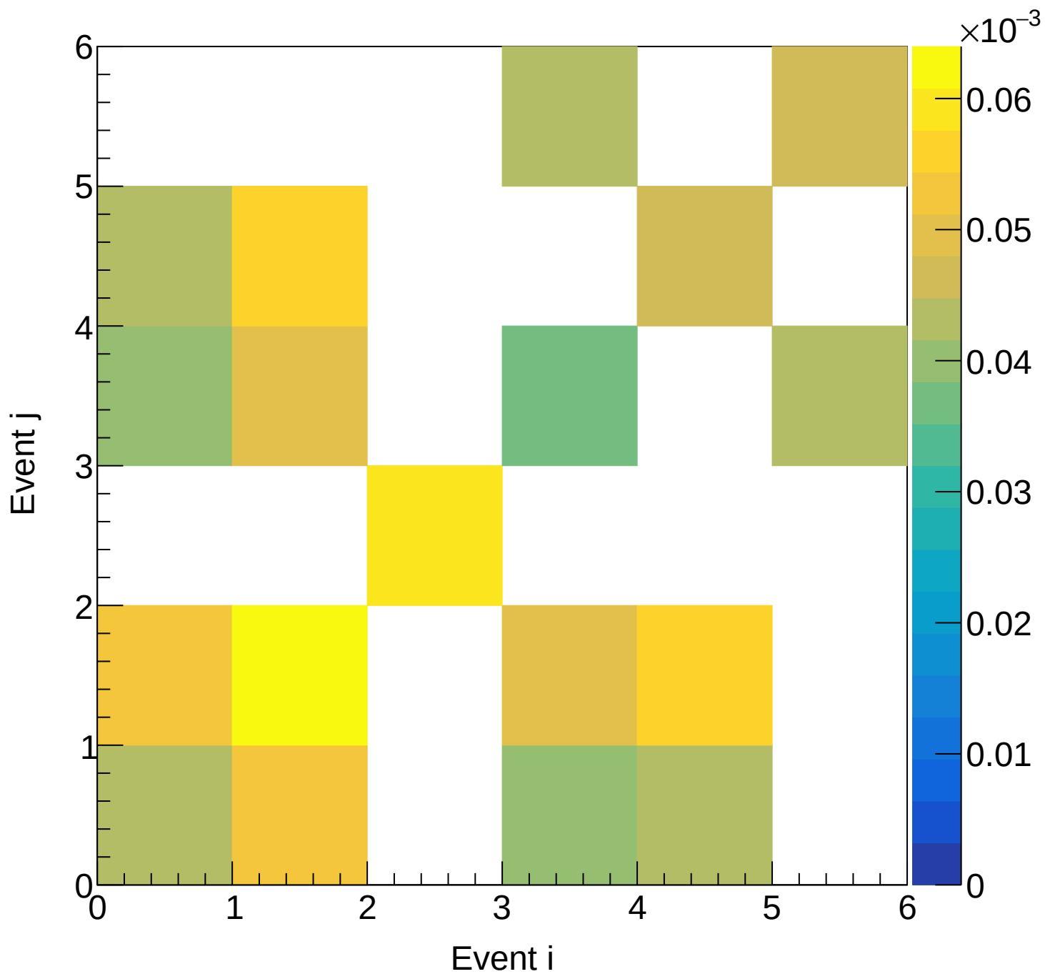
LH2 (mix) Covariance | M: [5.7, 6.0] xF: [0.10, 0.15)
