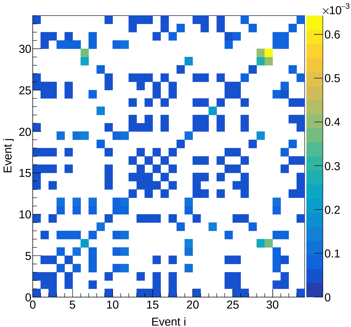
LH2 (mix) Covariance | M: [4.5, 4.8) xF: [0.15, 0.20)
