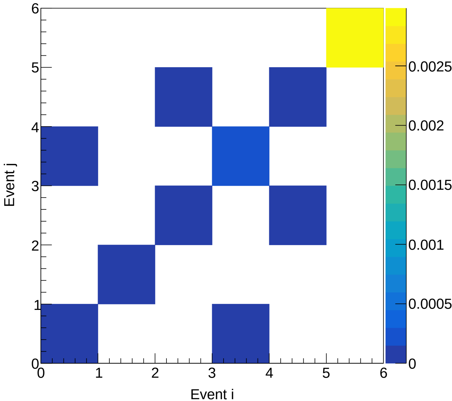
LH2 (mix) Covariance | M: [5.4, 5.7) xF: [0.15, 0.20)
