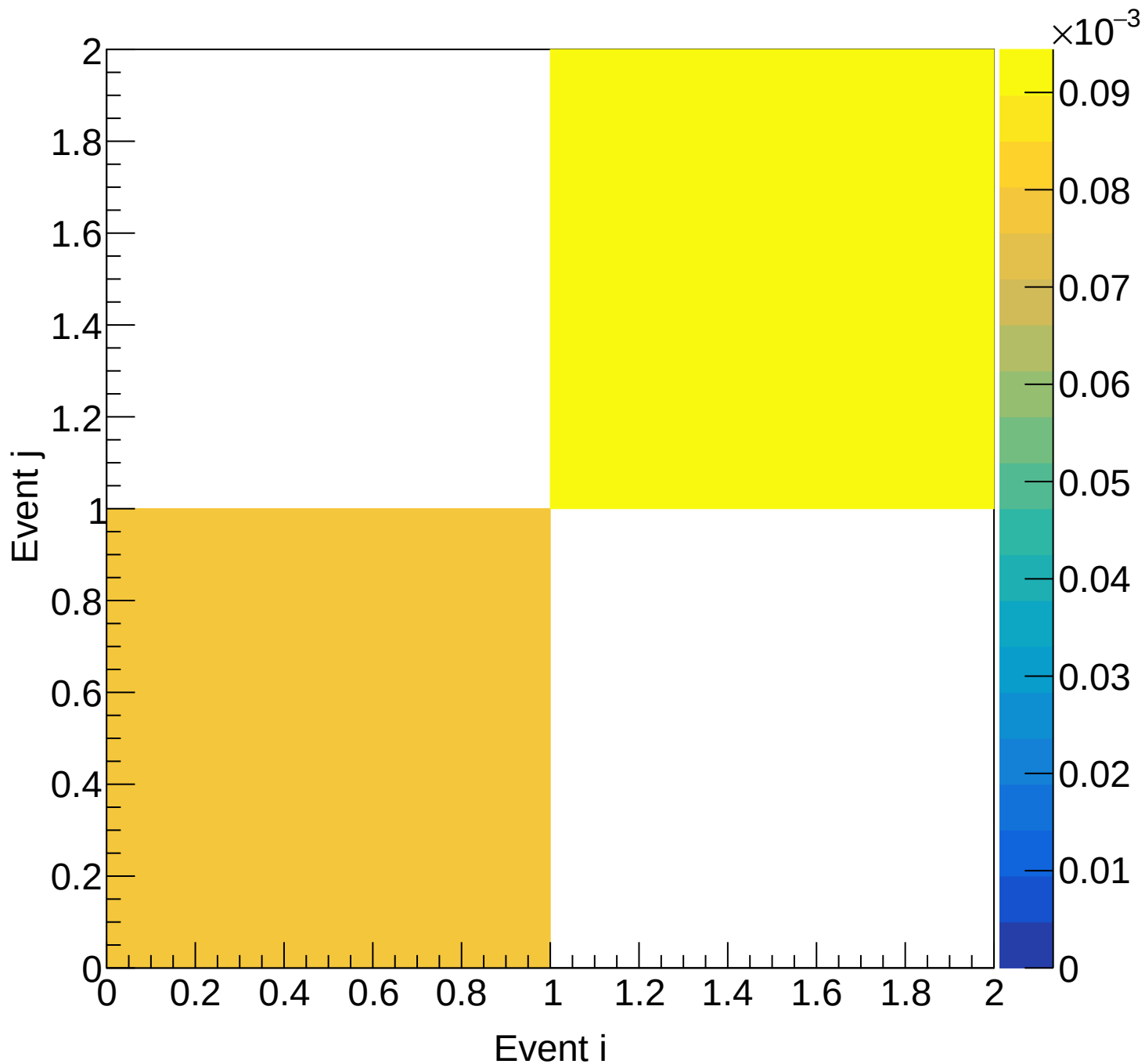
LH2 (mix) Covariance | M: [5.7, 6.0] xF: [0.15, 0.20]
