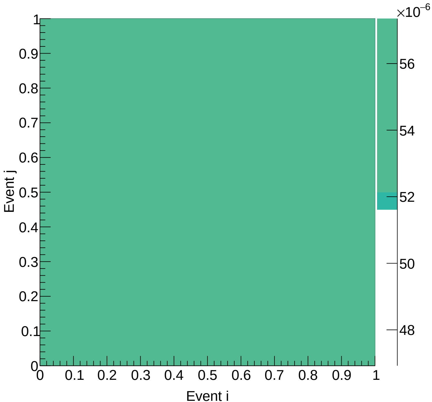
LH2 (mix) Covariance | M: [6.0, 6.3) xF: [0.15, 0.20)
