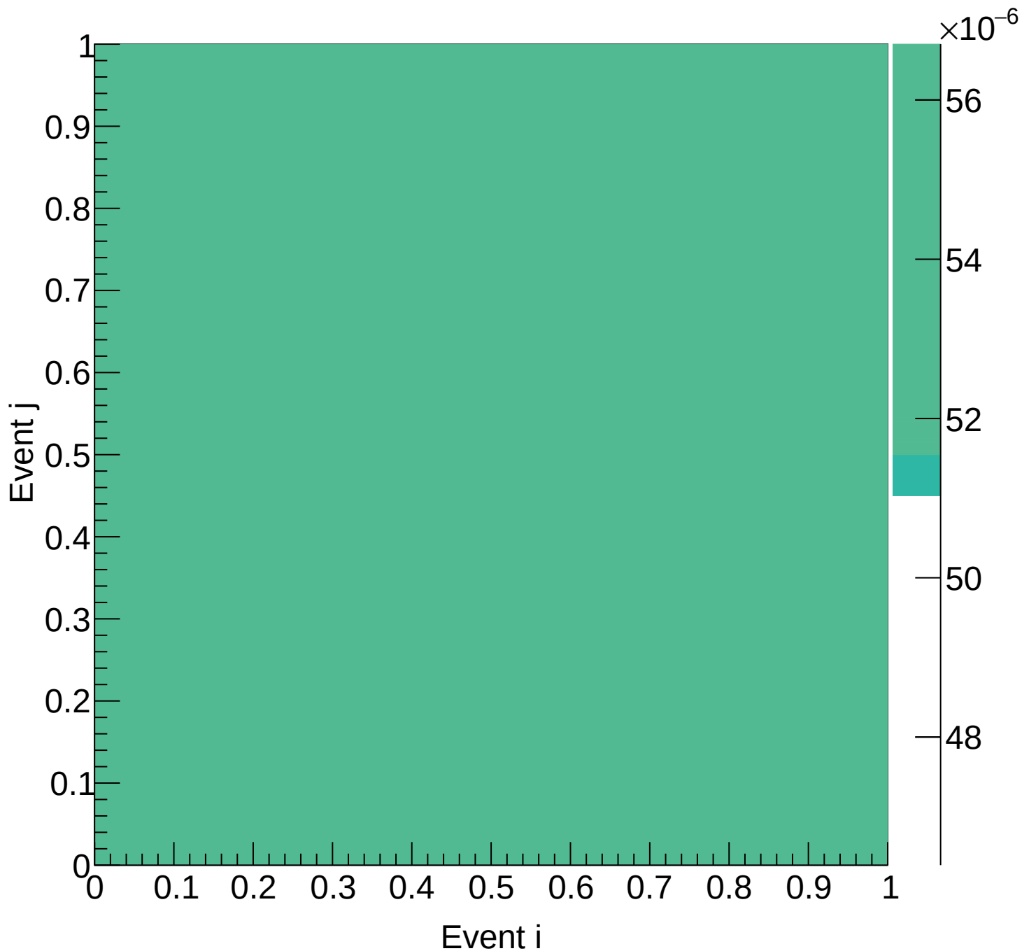
LH2 (mix) Covariance | M: [6.9, 7.5) xF: [0.20, 0.25)
