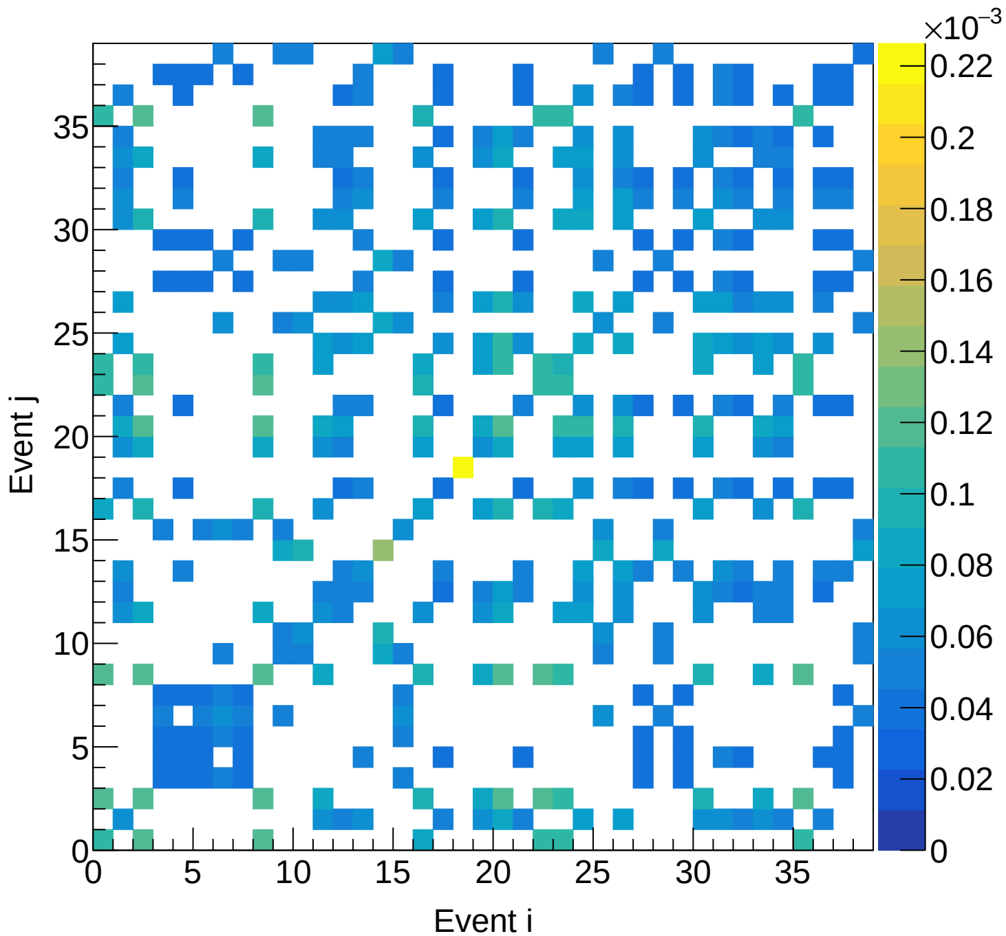
LH2 (mix) Covariance | M: [4.8, 5.1) xF: [0.20, 0.25)
