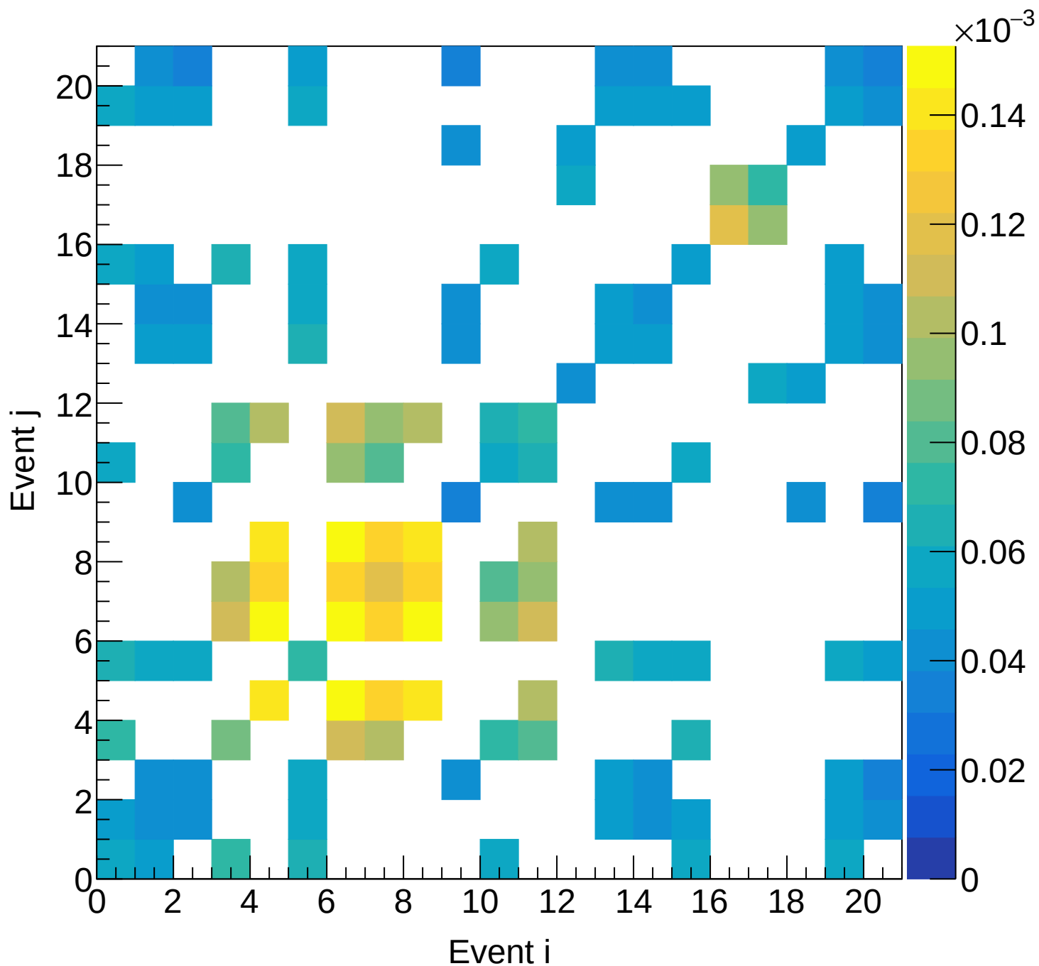
LH2 (mix) Covariance | M: [5.1, 5.4) xF: [0.20, 0.25)
