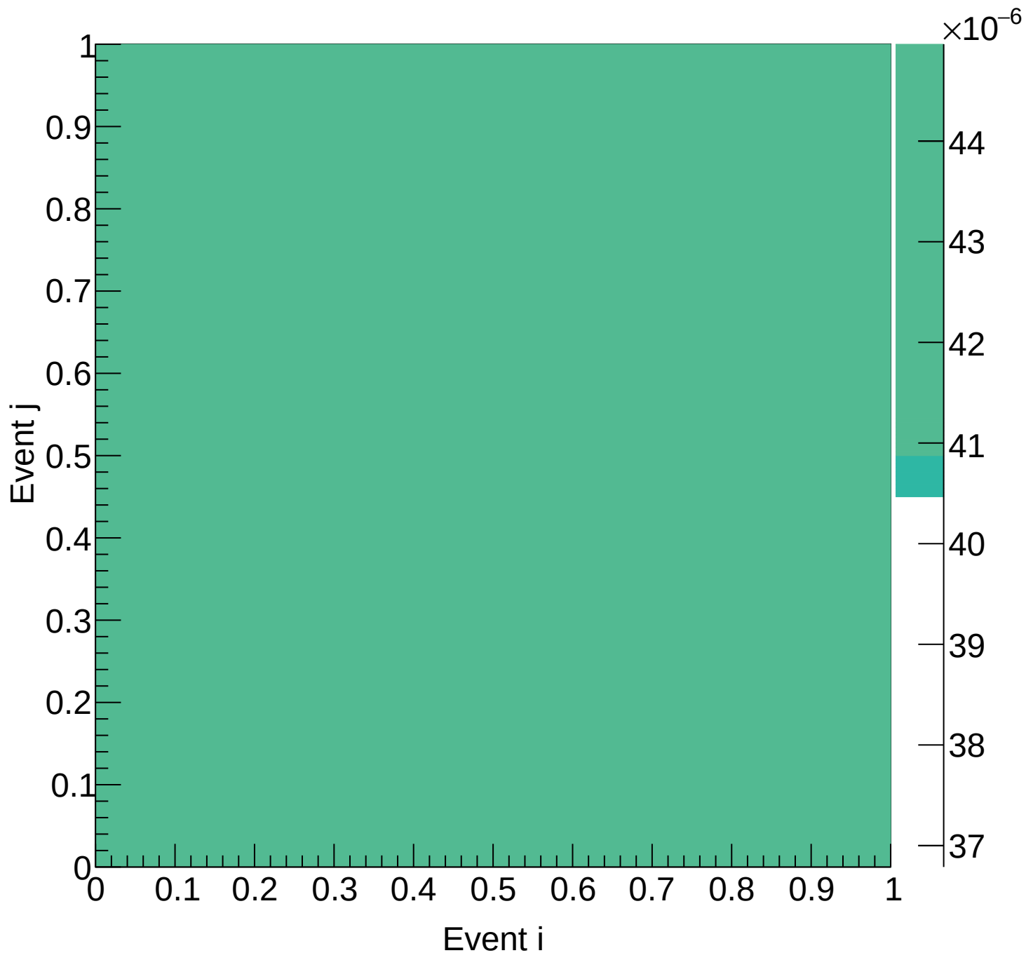
LH2 (mix) Covariance | M: [6.0, 6.3) xF: [0.20, 0.25)
