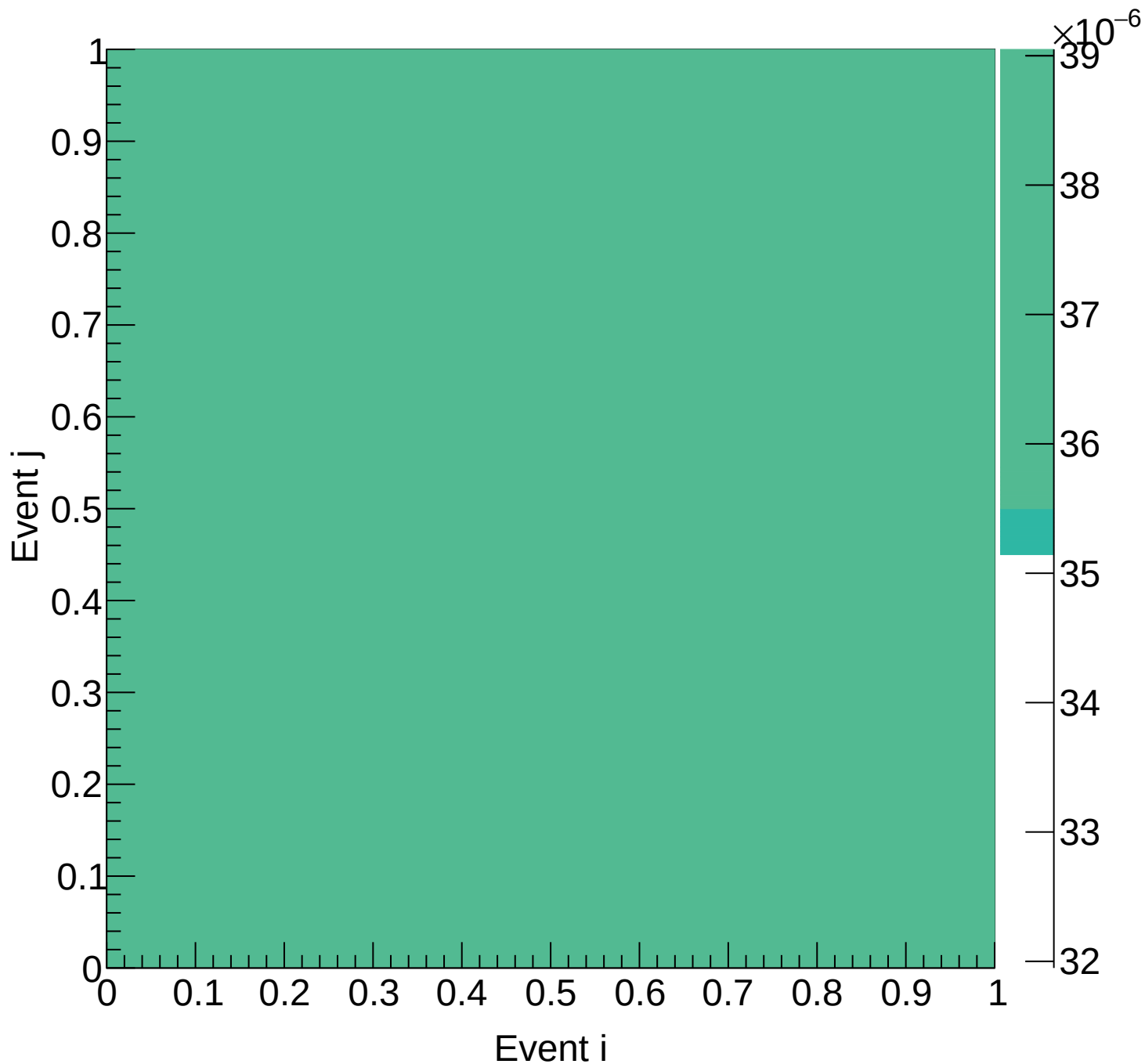
LH2 (mix) Covariance | M: [6.3, 6.6) xF: [0.20, 0.25)
