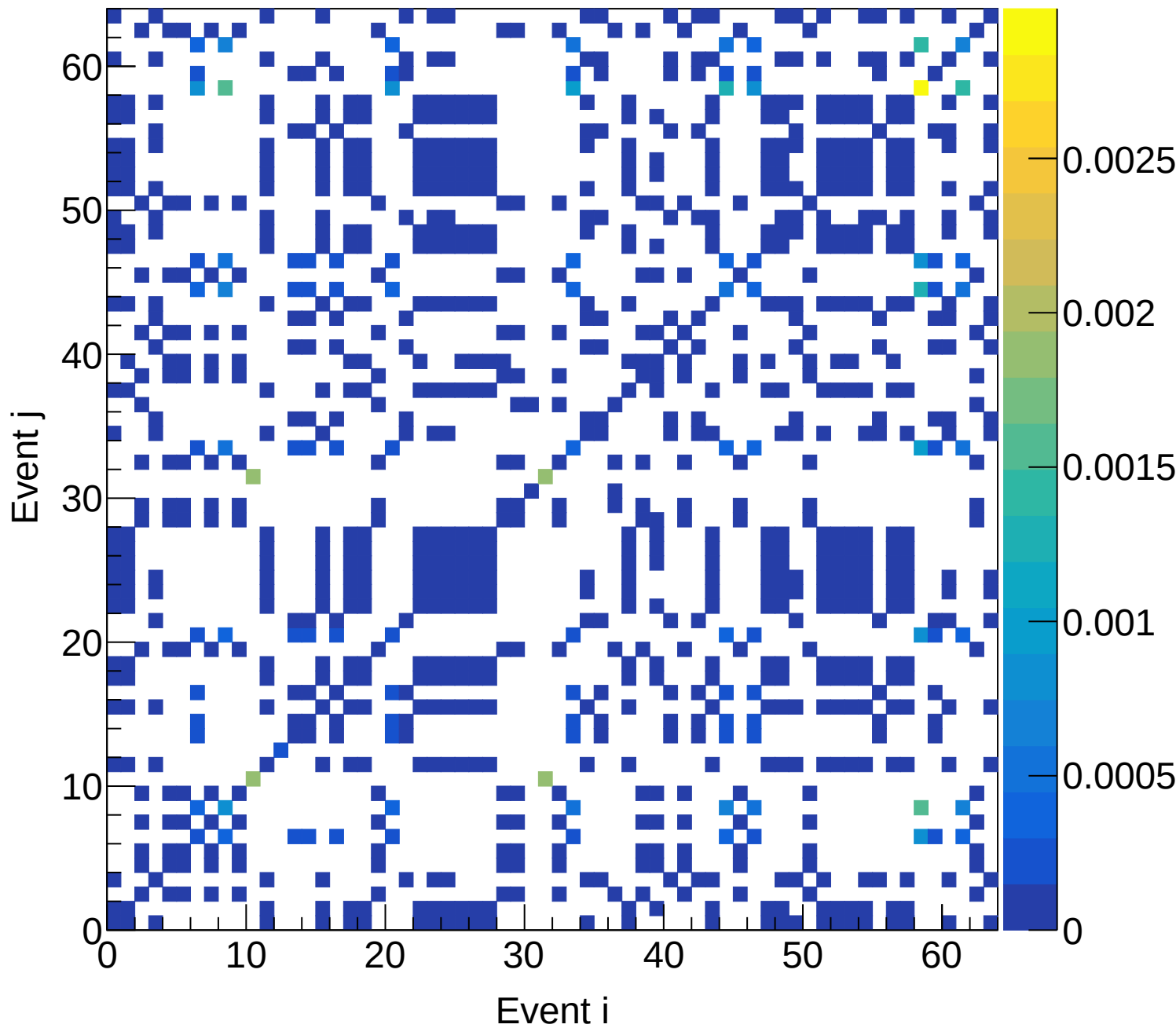
LH2 (mix) Covariance | M: [4.5, 4.8) xF: [0.25, 0.30)
