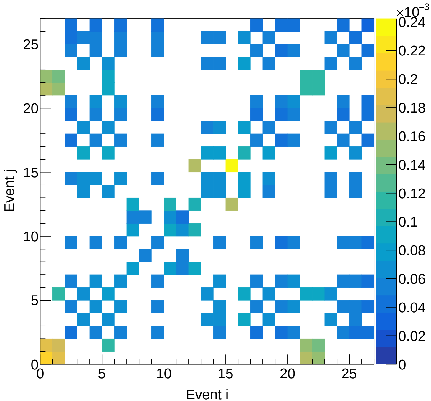
LH2 (mix) Covariance | M: [4.8, 5.1] xF: [0.25, 0.30]
