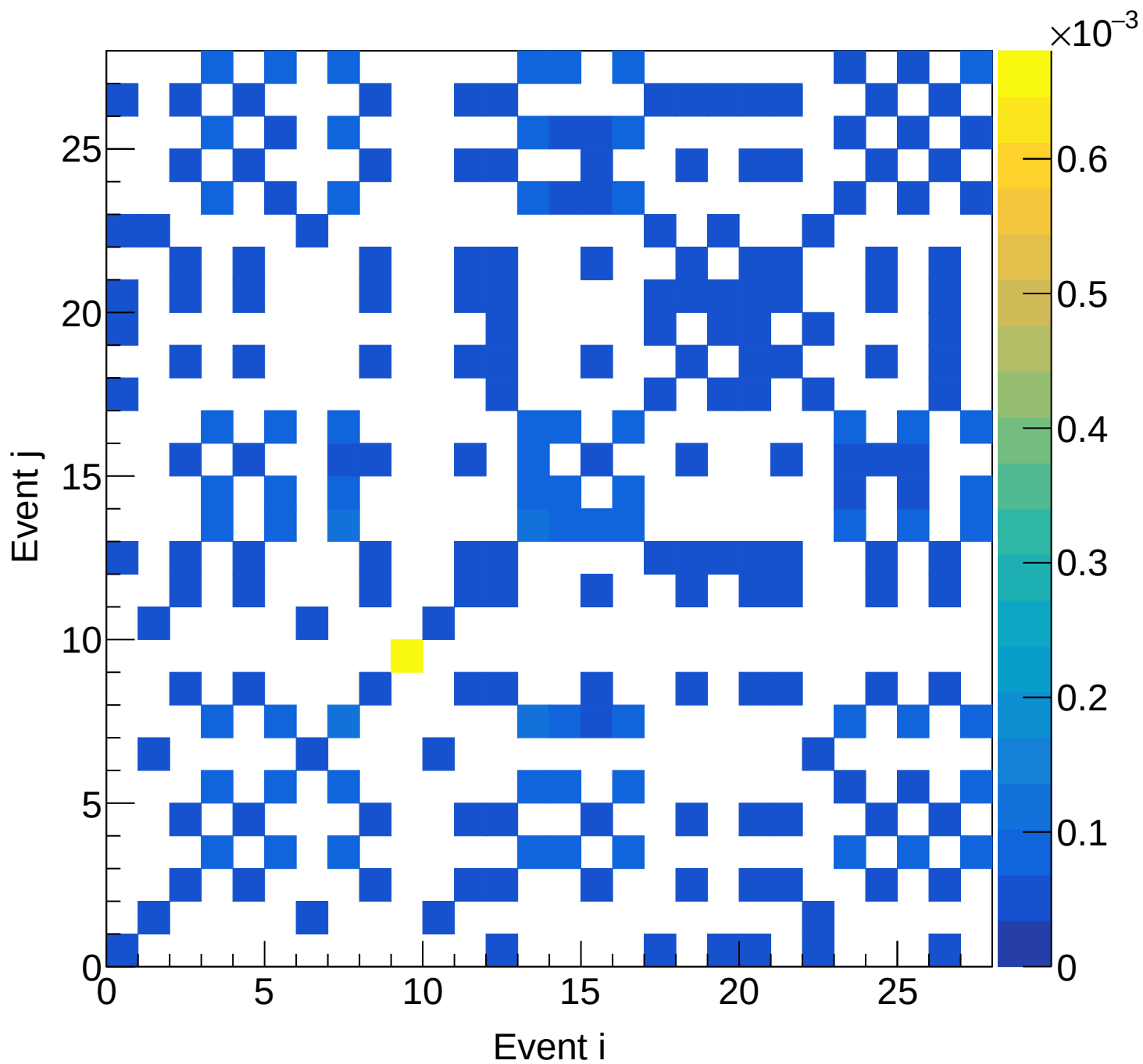
LH2 (mix) Covariance | M: [5.1, 5.4) xF: [0.25, 0.30)
