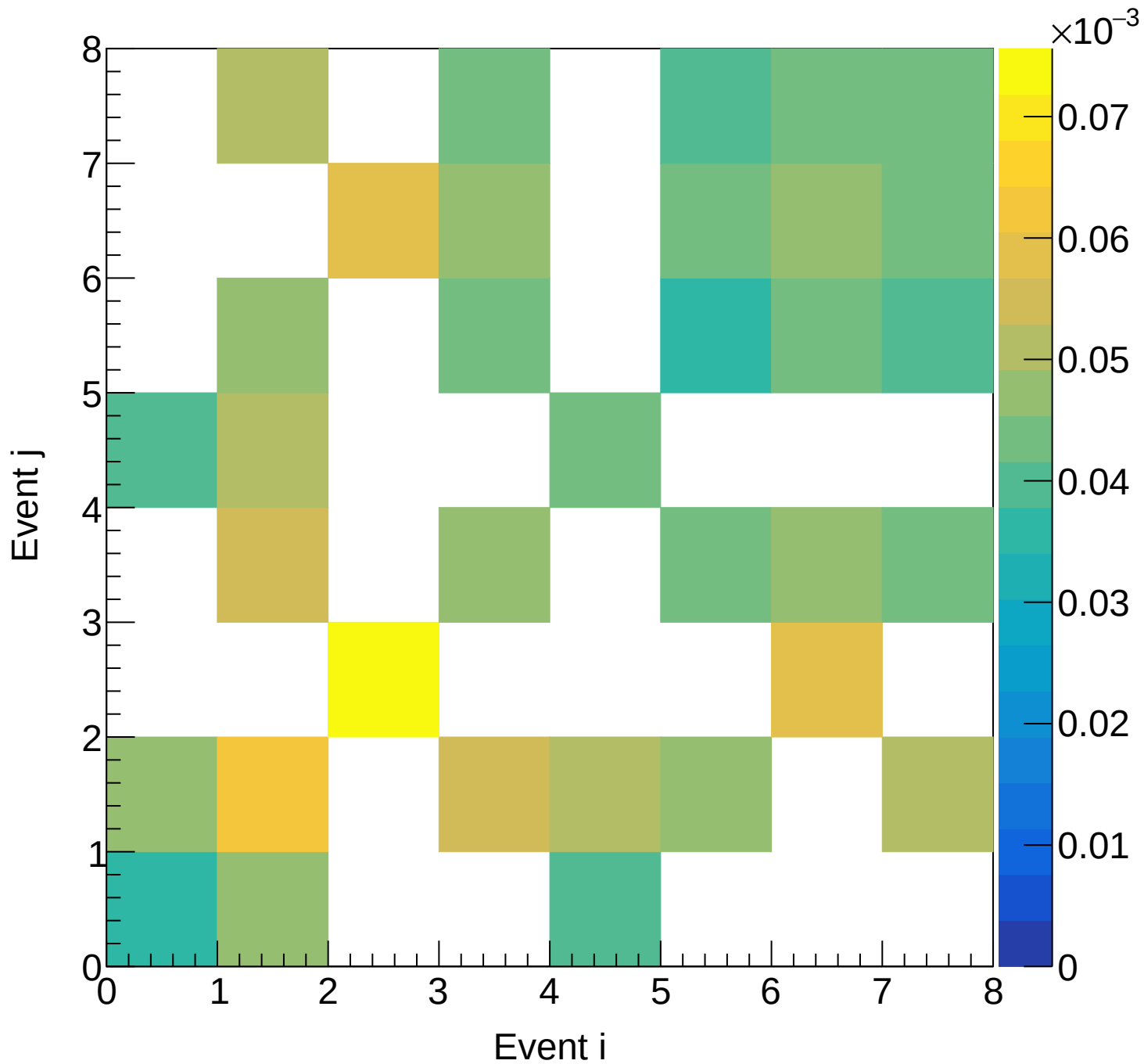
LH2 (mix) Covariance | M: [5.7, 6.0) xF: [0.25, 0.30)
