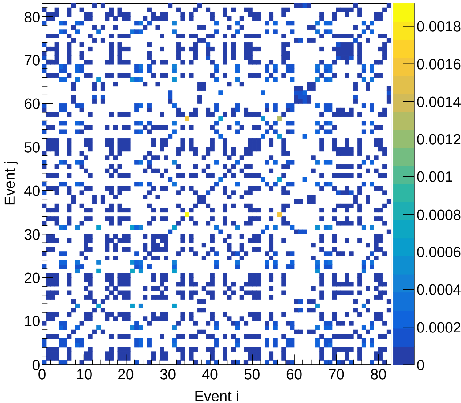
LH2 (mix) Covariance | M: [3.9, 4.2) xF: [0.30, 0.35)
