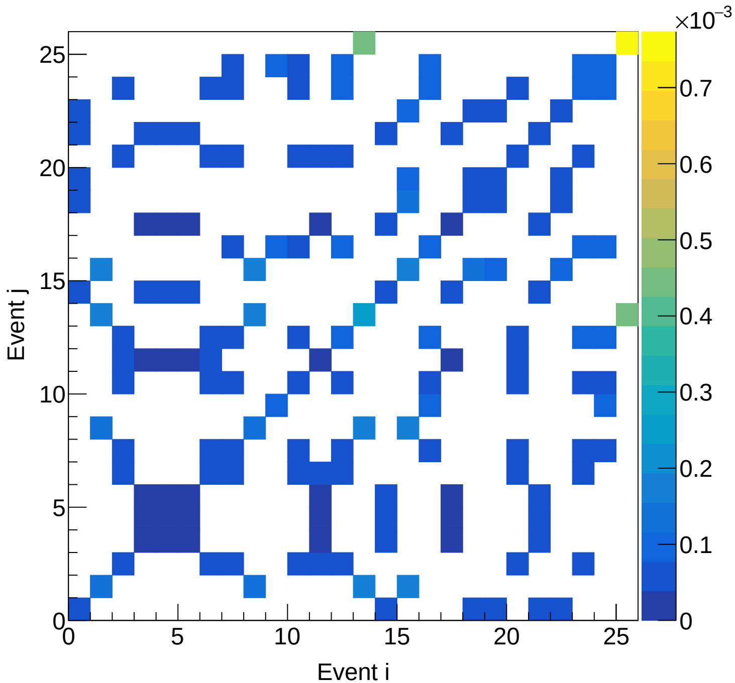
LH2 (mix) Covariance | M: [4.8, 5.1) xF: [0.30, 0.35)
