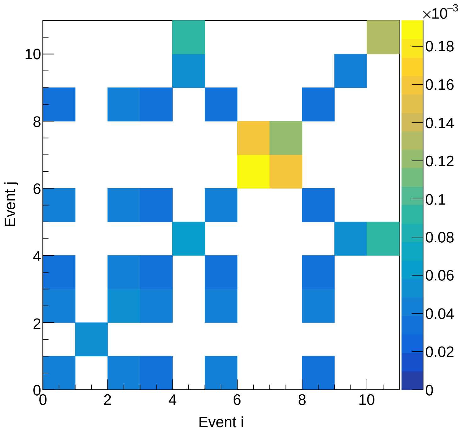
LH2 (mix) Covariance | M: [5.1, 5.4) xF: [0.30, 0.35)
