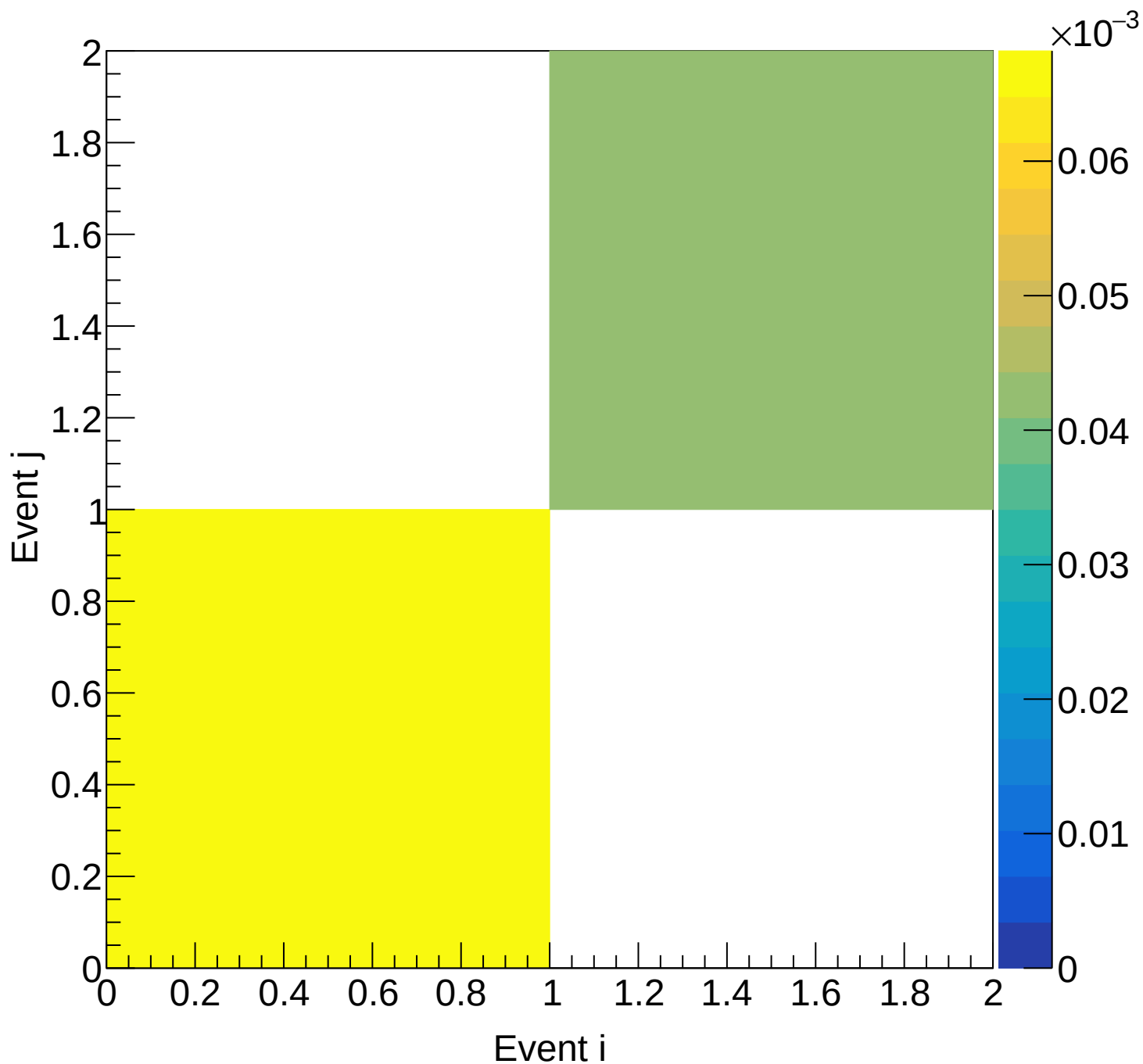
LH2 (mix) Covariance | M: [6.0, 6.3) xF: [0.30, 0.35)
