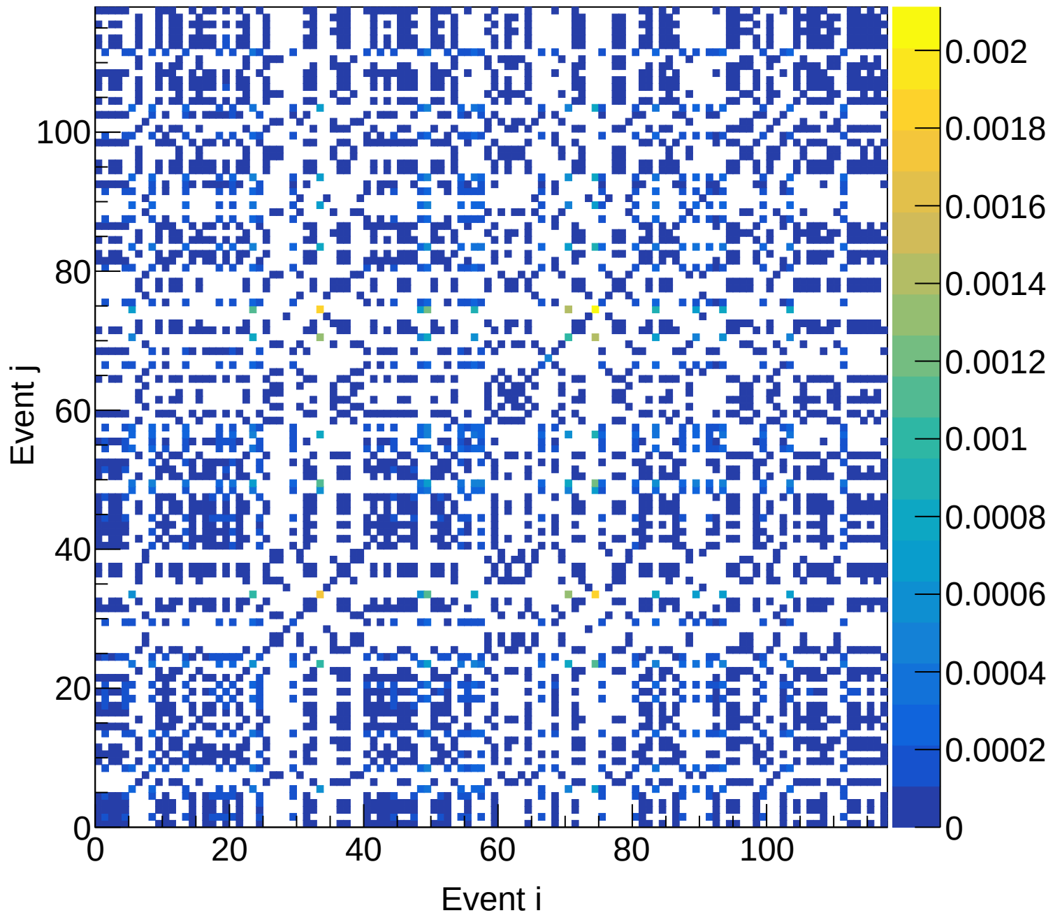
LH2 (mix) Covariance | M: [3.9, 4.2] xF: [0.35, 0.40)
