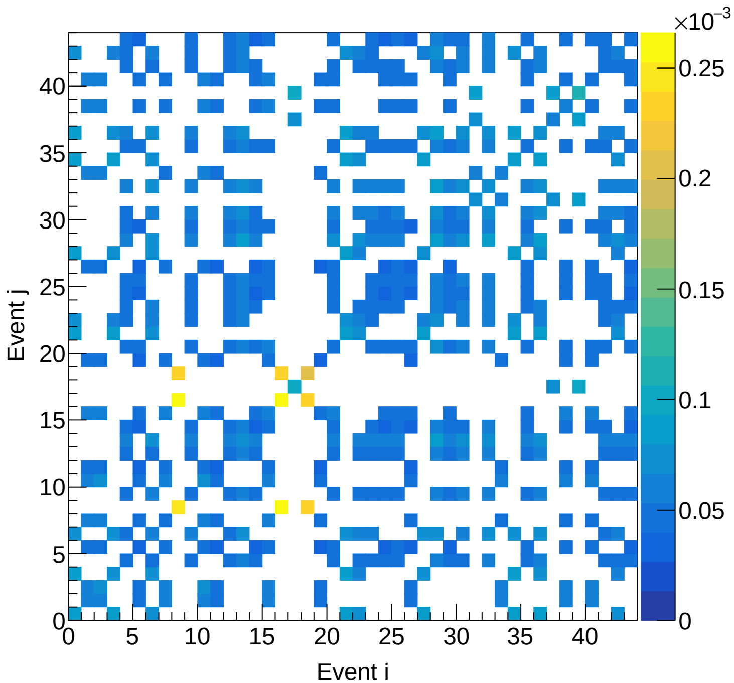
LH2 (mix) Covariance | M: [4.5, 4.8) xF: [0.35, 0.40)
