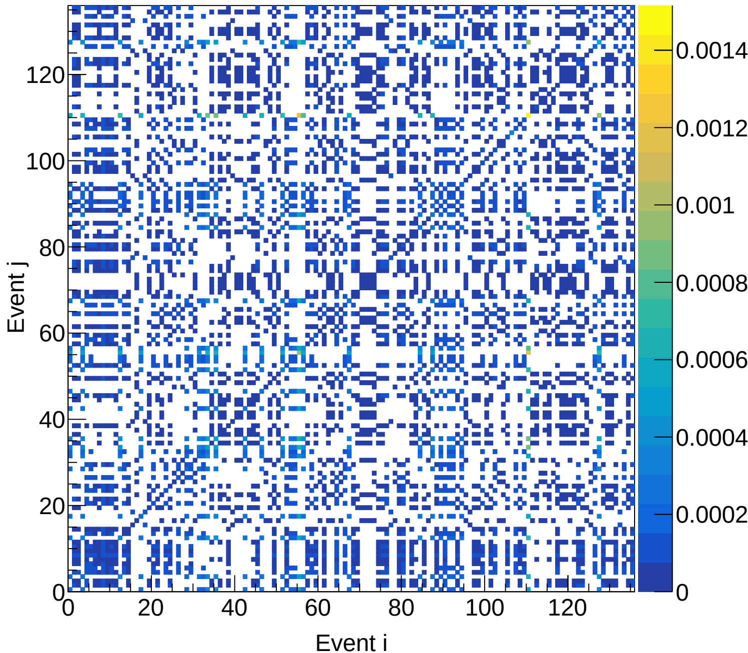
LH2 (mix) Covariance | M: [3.9, 4.2) xF: [0.40, 0.45)
