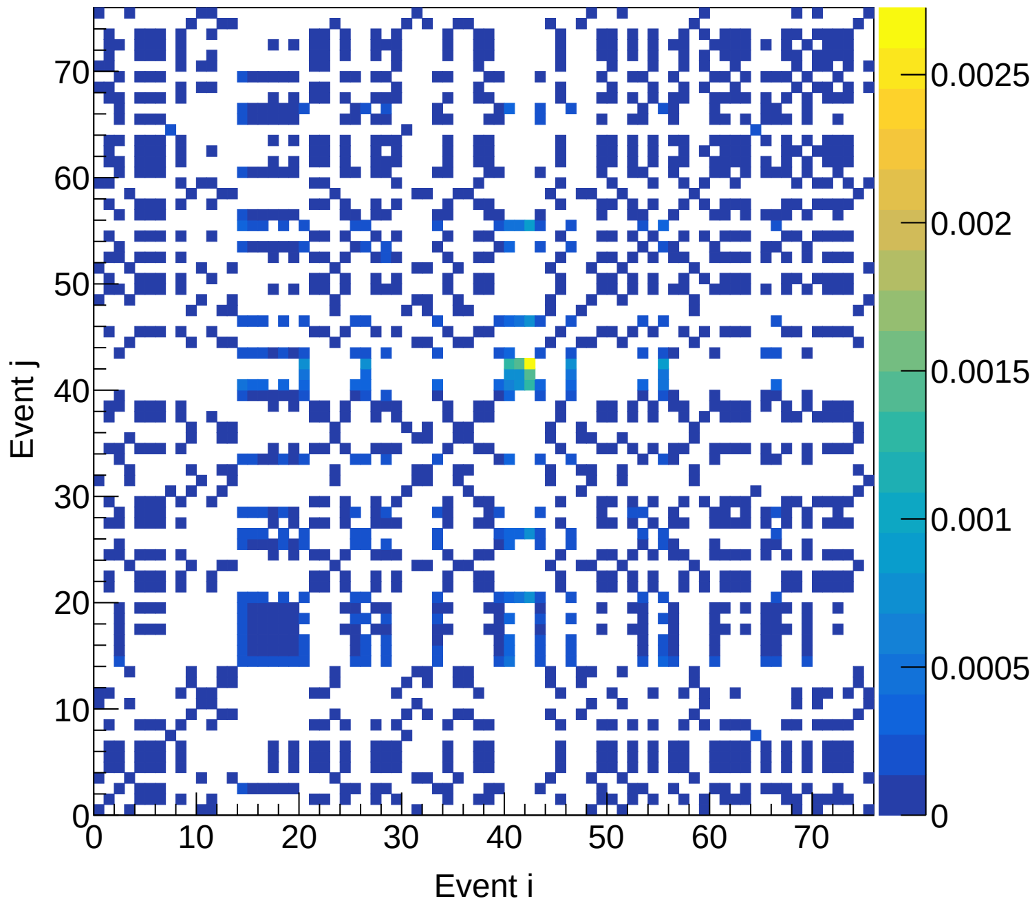
LH2 (mix) Covariance | M: [4.2, 4.5) xF: [0.40, 0.45)
