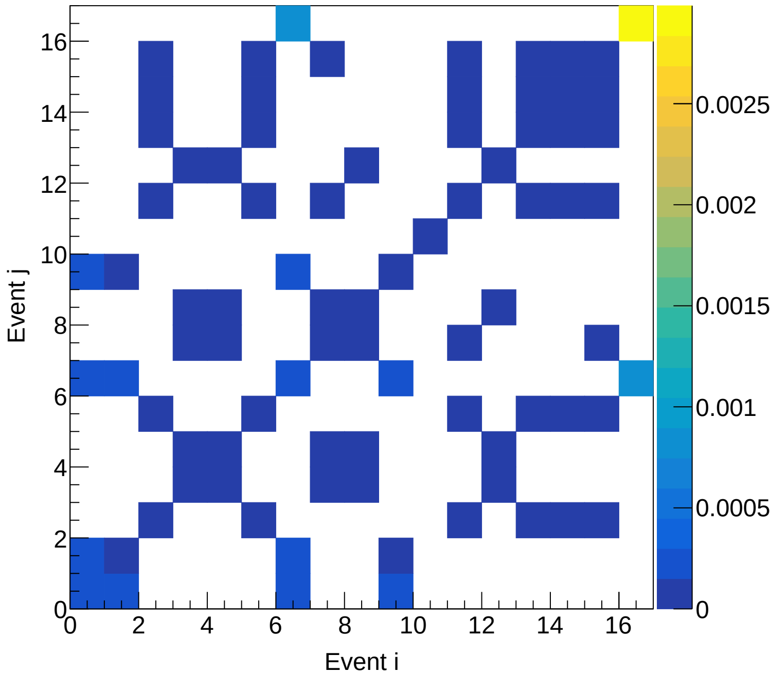
LH2 (total) Covariance | M: [4.8, 5.1) xF: [-0.05, 0.00)
