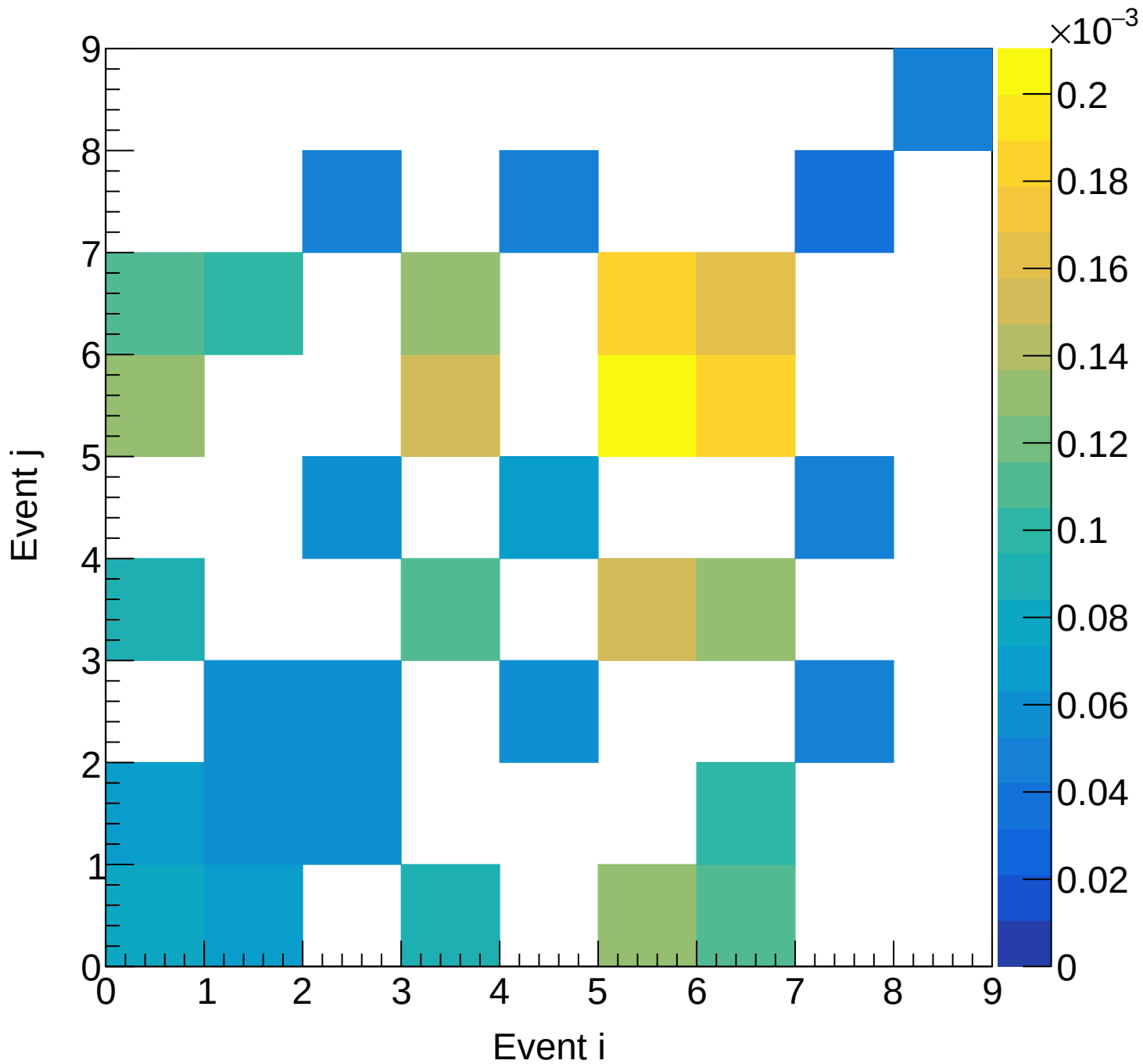
LH2 (total) Covariance | M: [6.6, 6.9] xF: [-0.05, 0.00)
