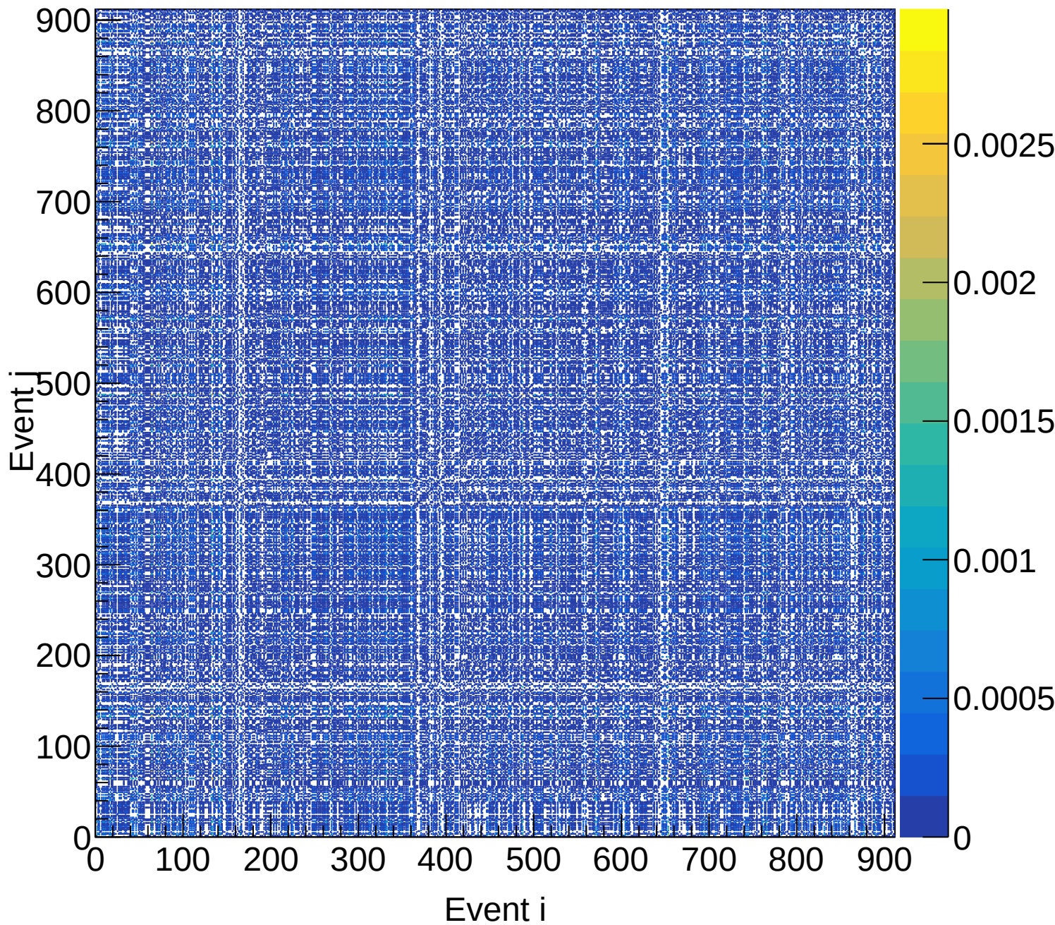
LH2 (total) Covariance | M: [3.9, 4.2) xF: [0.45, 0.50)
